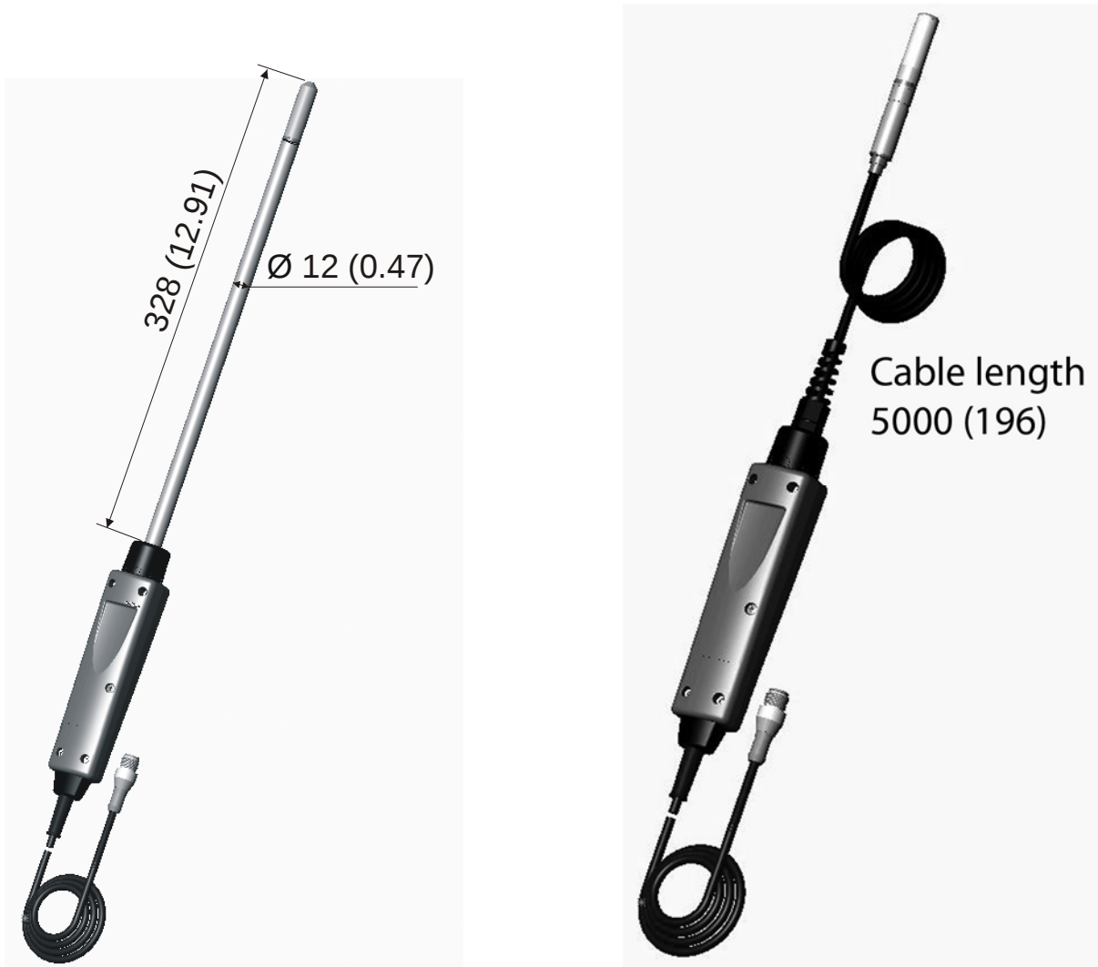
HMP76 Probe
