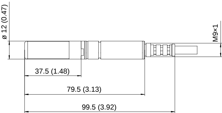
HMP77 Probe
