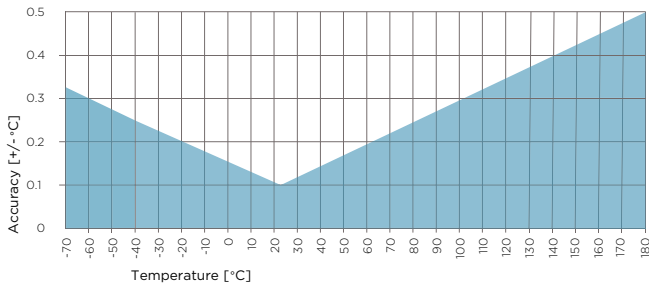
HMP7 Temperature Measurement Accuracy over Full Range (Including Non-Linearity and Repeatability)
