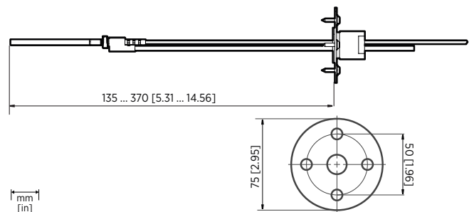
Optional Duct Kit 215003 Dimensions
