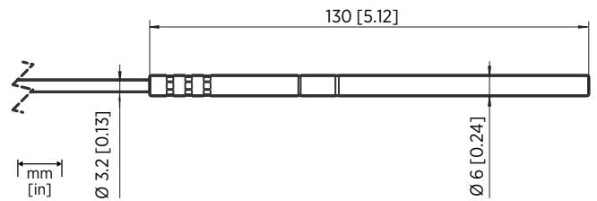
TMP1 Probe Head Dimensions
