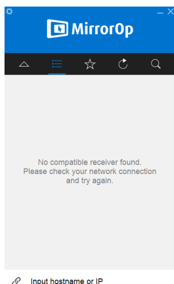
MirrorOp Sender
