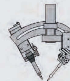
Solder feeder retracts to allow enough space for tip cleaning
