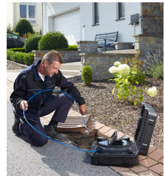
The 100' push rod and the pan- and tiltable camera head 1.5" make sure nothing in the house supply line remains hidden from your view.
