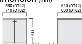
OT models
