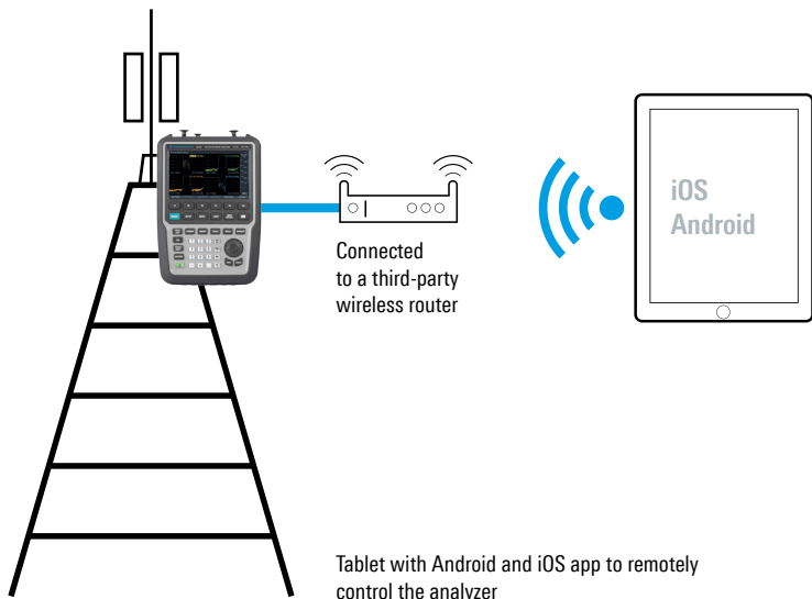
Application example of wireless remote operation via tablet
