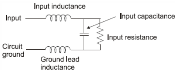
Figure 2. Generic probe input equivalent circuit.
