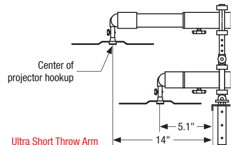
Ultra Short Throw Arm
