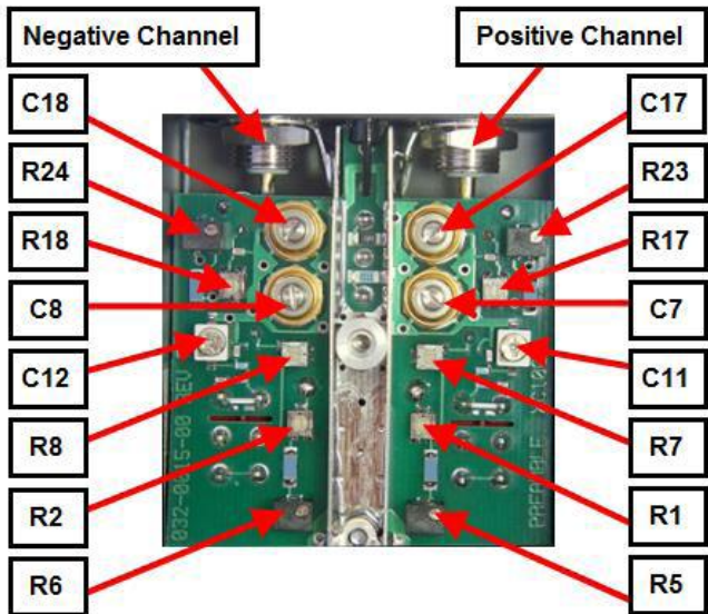
Figure 1, The DXC100A Board Layout
