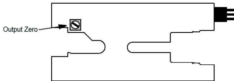
Figure 7 Adjustment Location S/N 1000 and higher
