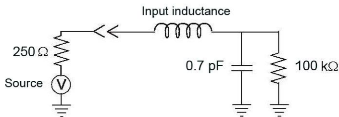
Figure 3 Probe input equivalent circuit
