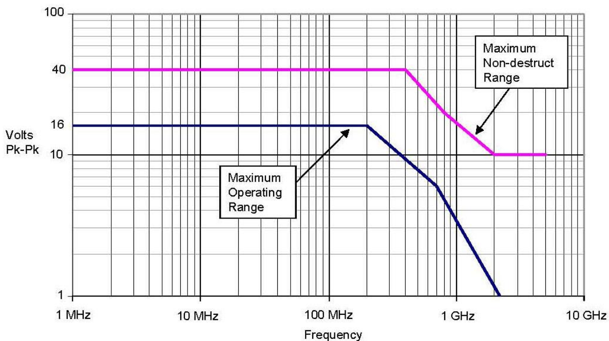
Figure 9 Input Voltage vs. Frequency
