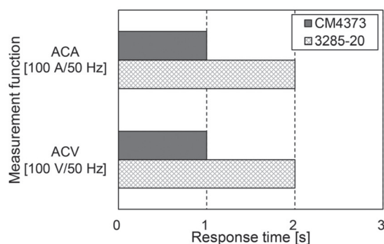
Fig. 6. Difference in response time vs. 3285-20 (legacy product).
