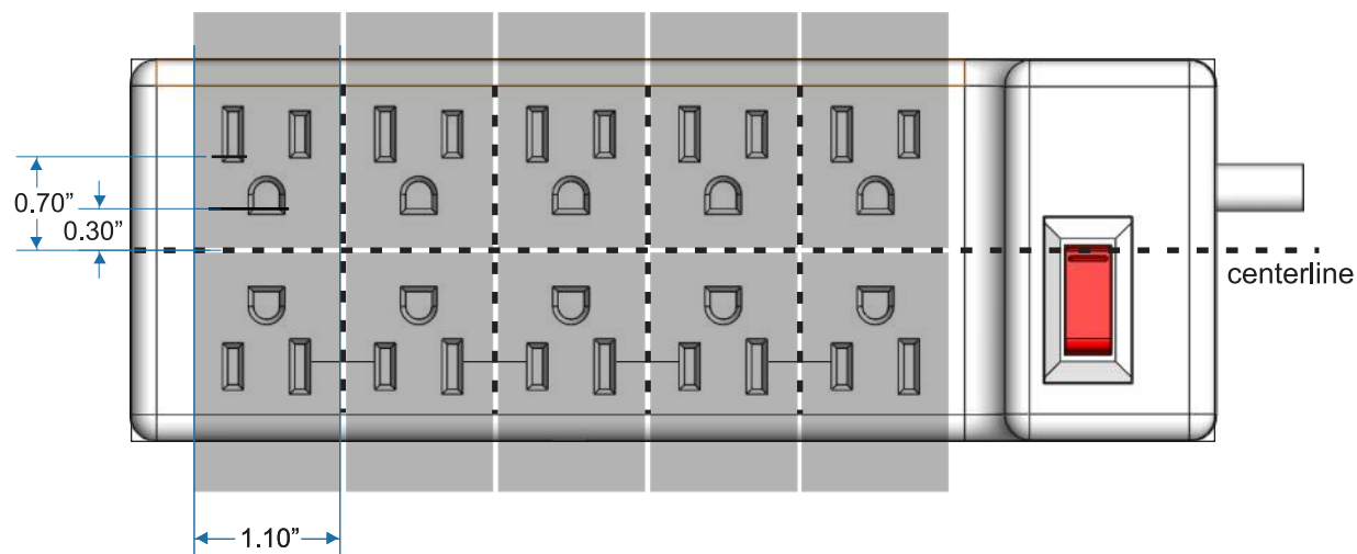
10 Outlet Power Strip
