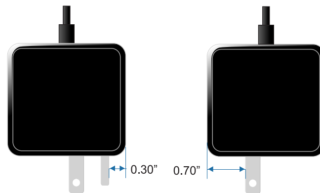
Fitting power adapters onto 10 Outlet Power Strip
