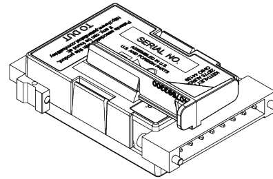
Figure 3: Installing the support bracket for use in channel A
