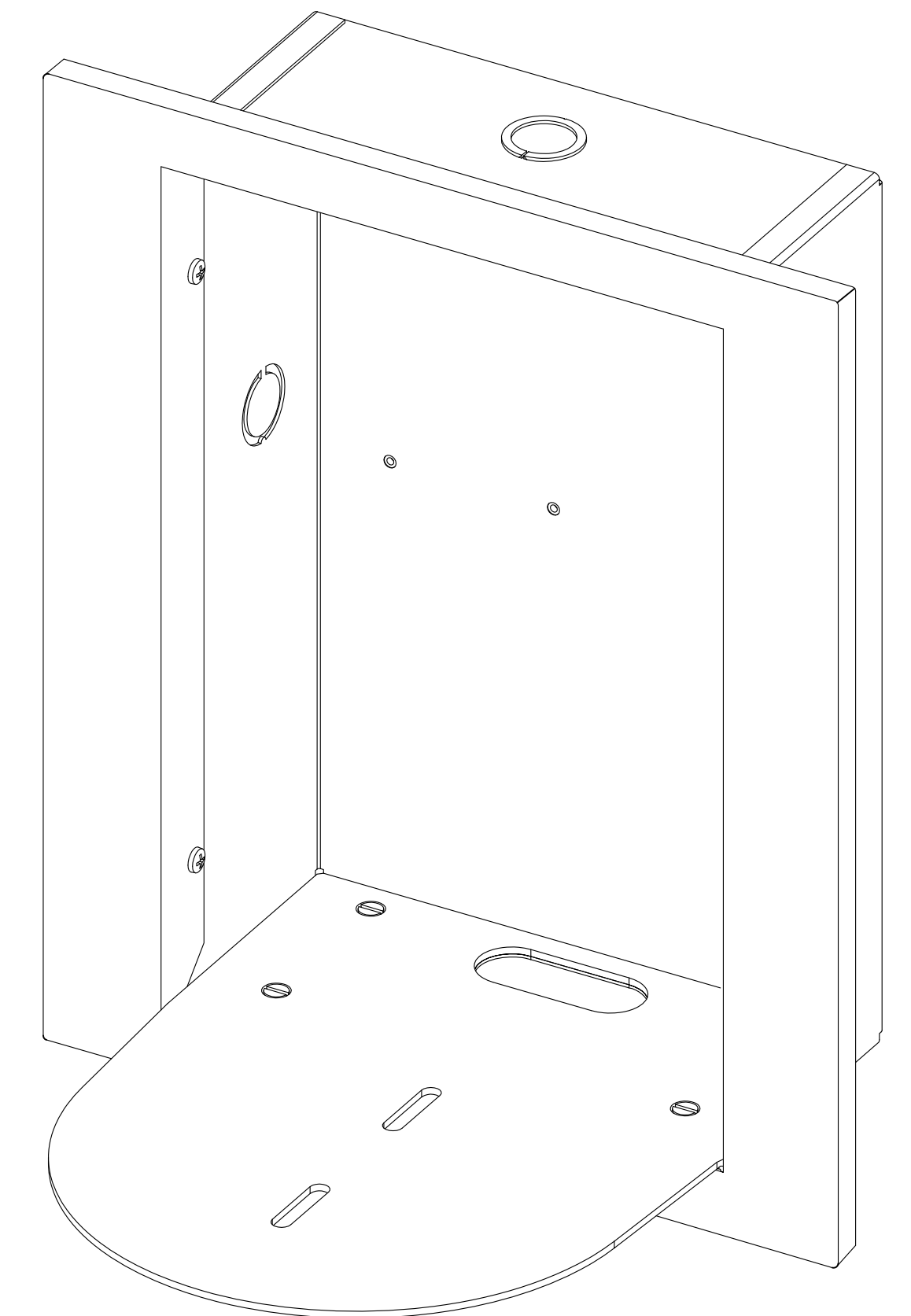
CAMERA BOX, PLATFORM AND FRAME ISO VIEW (NO SCALE)
