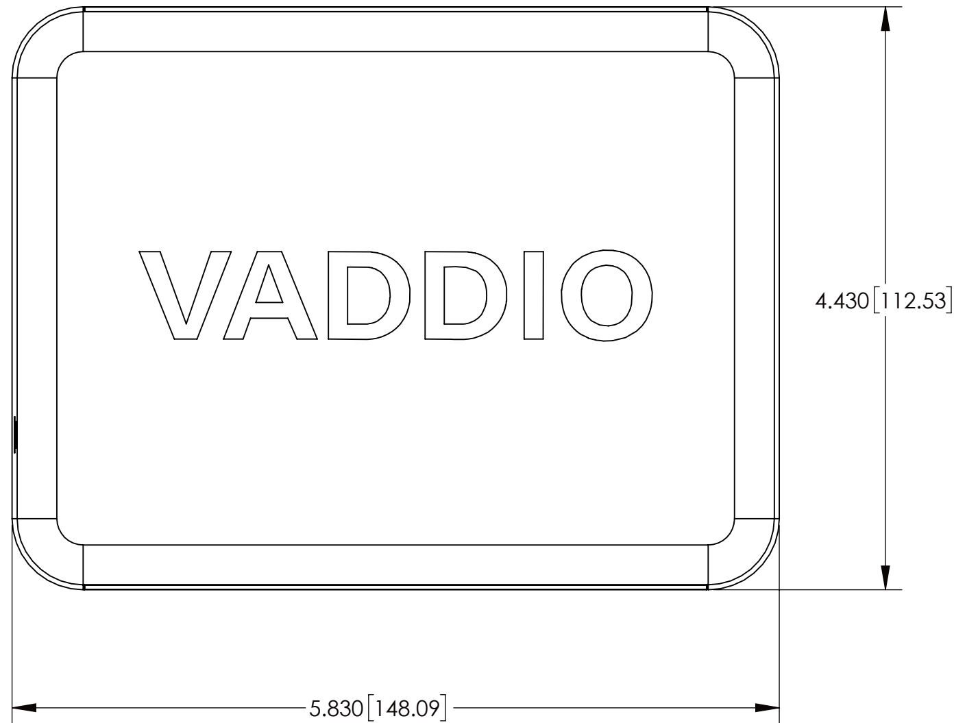
TOP VIEW
