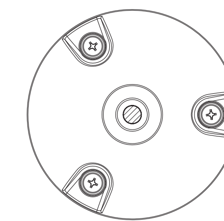
SECTION A - A CEILING MicPOD TOP VIEW
