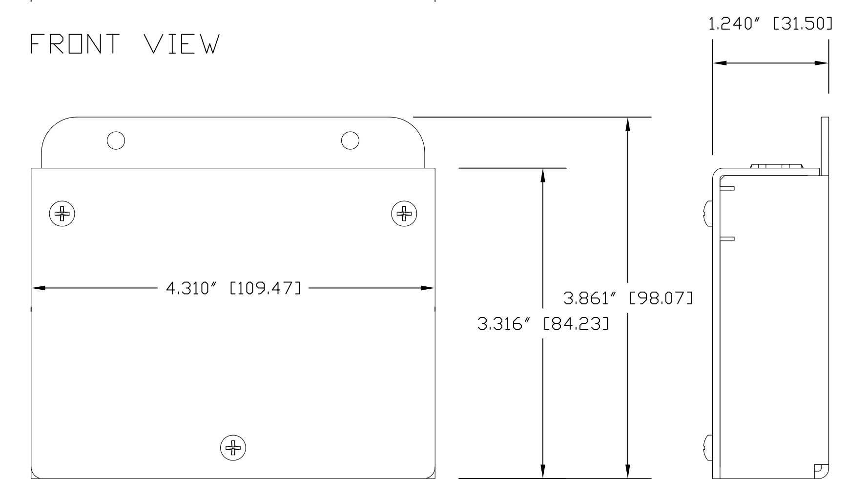
SIDE VIEW
