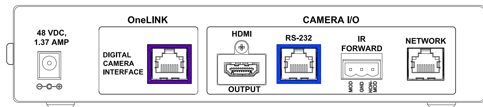
REAR VIEW
