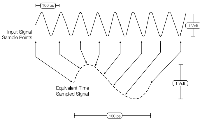
Figure 25. Basic sampling, showing sample points are connected by interpolation to produce a continuous waveform.
