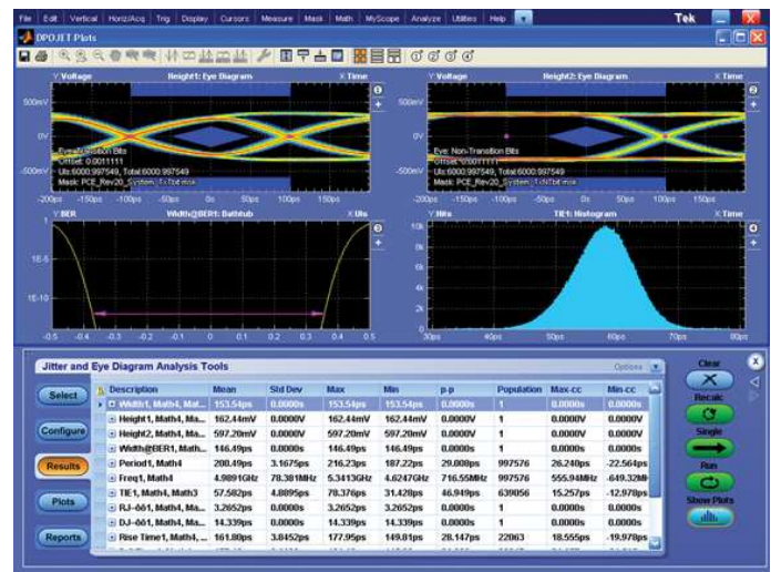
Figure 54. Analysis software packages are specifically designed to meet jitter and eye measurement needs of today's high-speed digital designers.
