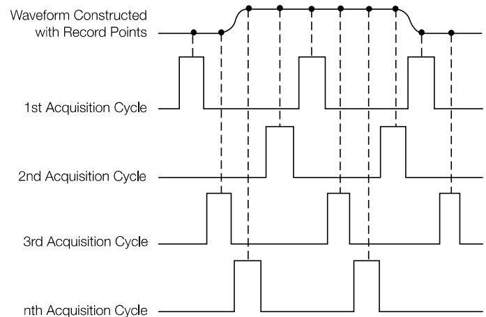
Figure 30. Some oscilloscopes use equivalent-time sampling to capture and display very fast, repetitive signals.
