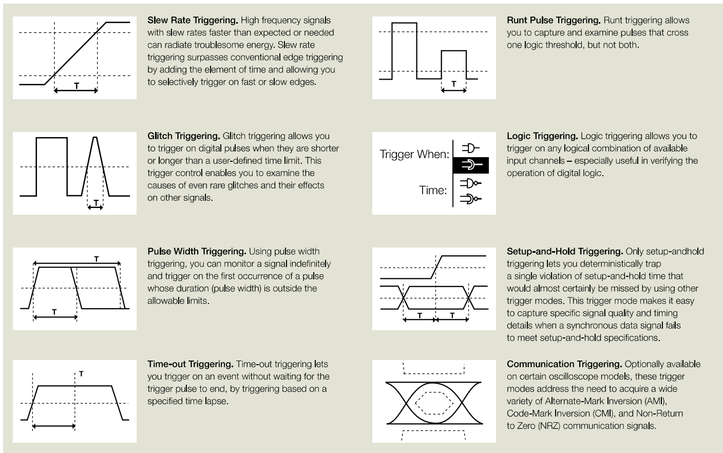
Figure 34. Common trigger types.
