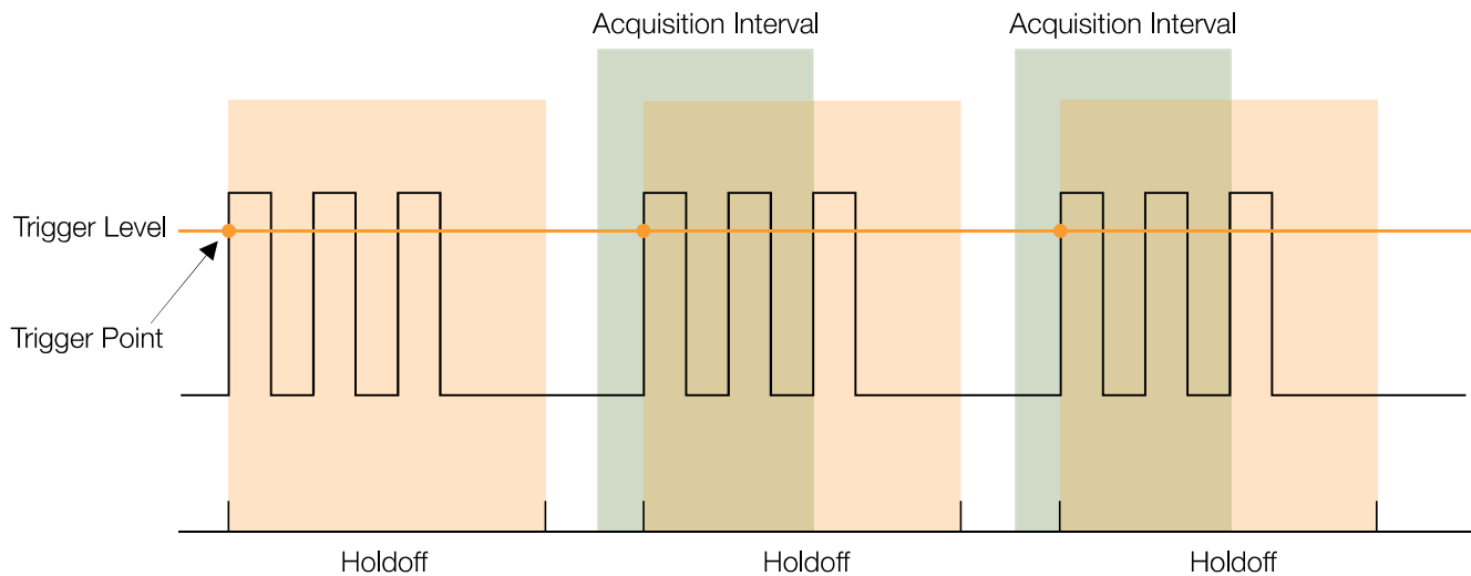
Figure 36. Trigger holdoff.
