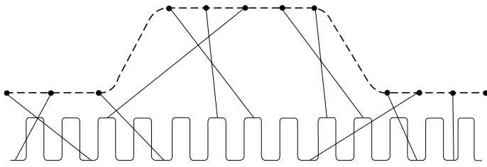
Figure 31. In random equivalent-time sampling, the sampling clock runs asynchronously with the input signal and the trigger.
