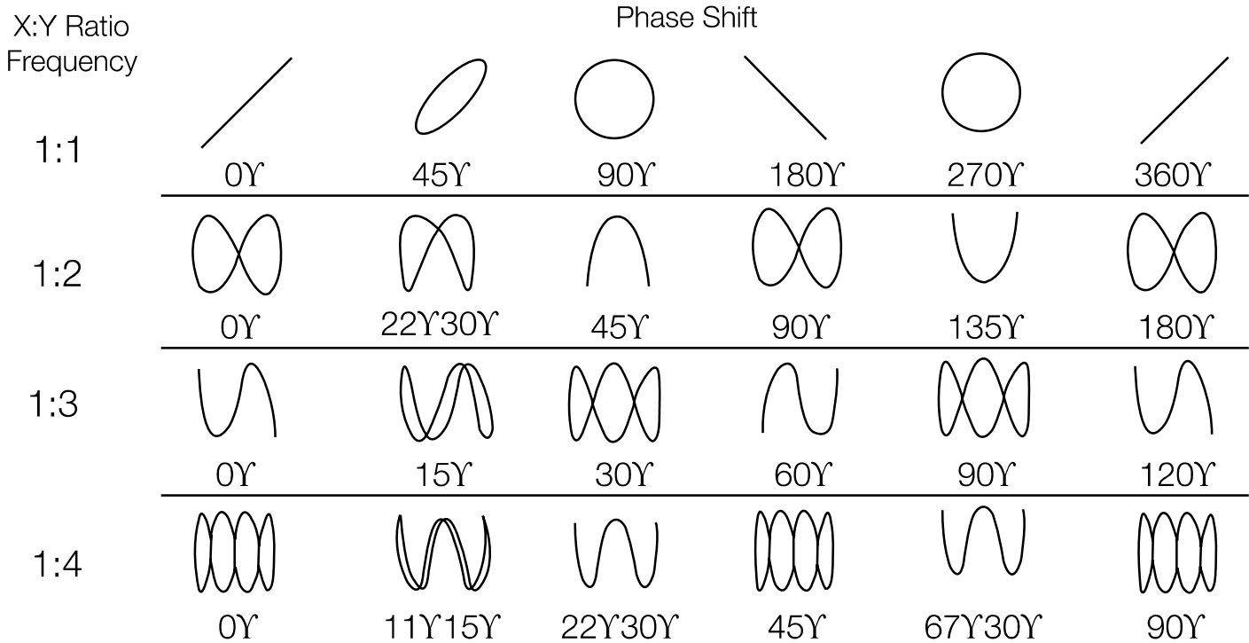
Figure 70. Lissajous patterns.
