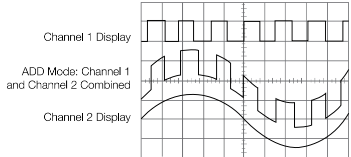
Figure 38. Adding channels.
