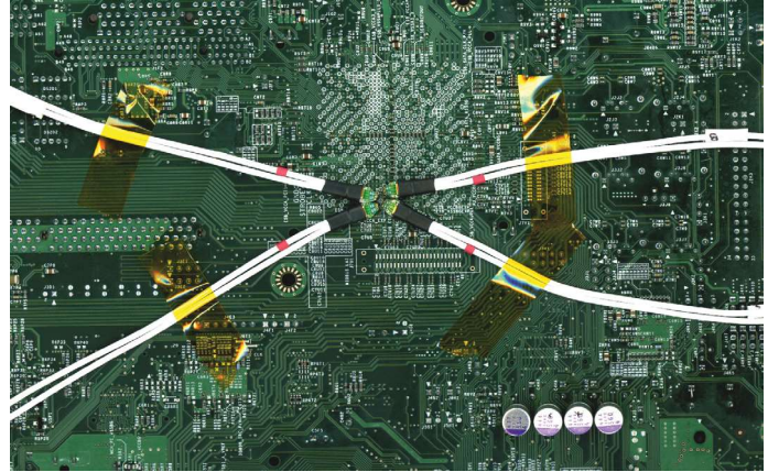
Figure 39. Dense devices and systems require small form factor probes.
