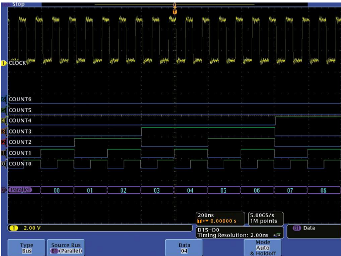
Figure 56. Automatically trigger, decode, and search on clocked and unclocked parallel bus data.
