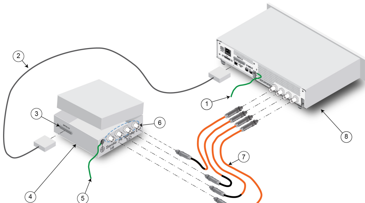
Figure 6: Physical four-wire connections to a test fixture with SHV connectors
