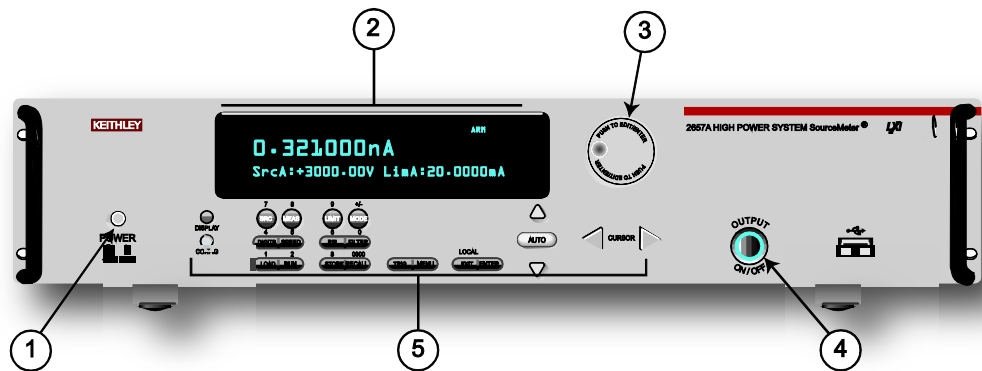
Figure 14: Front panel
