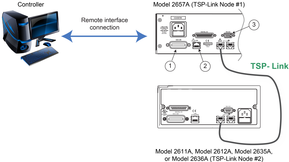
Figure 38: Remote interface and TSP-Link communications setup
