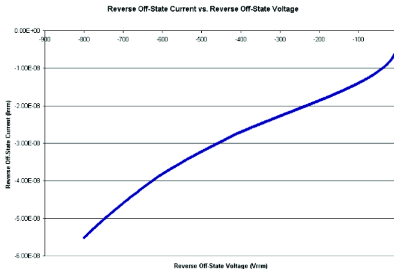
Figure 42: Sample output Vrrm
