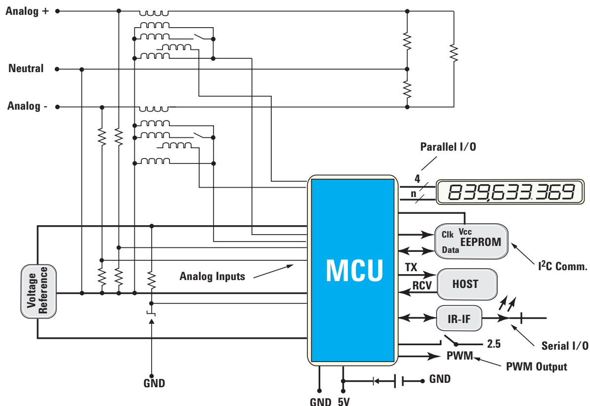
Figure 2. Typical MCU-based embedded design.
