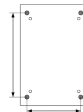
Fig. 2 - Mounting Hole Pattern C-C
