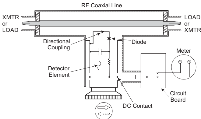
Figure 2 Schematic
