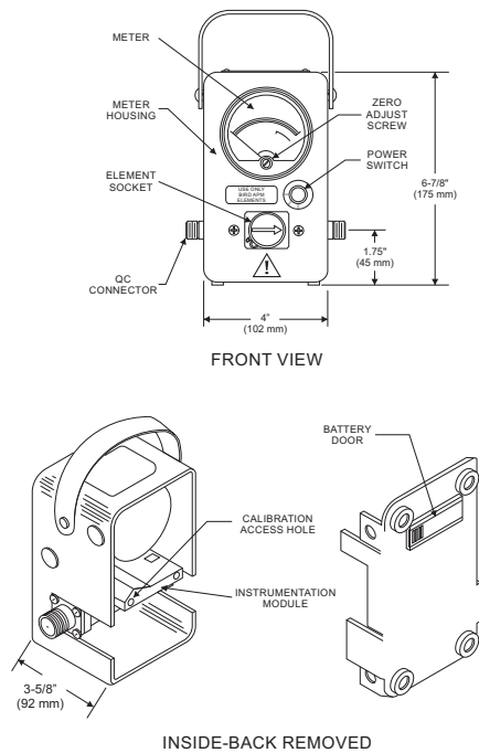
Figure 1 Outline Drawing
