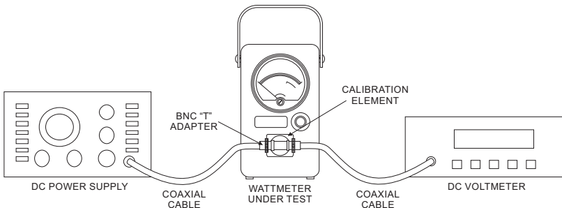
Figure 11 Calibration Setup
