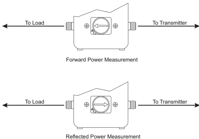
Figure 7 Element Direction
