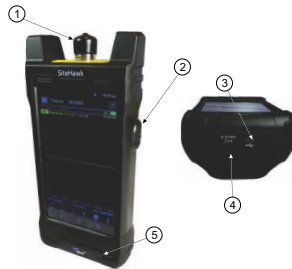
Figure 1 SK-4500 Connectors and Ports
