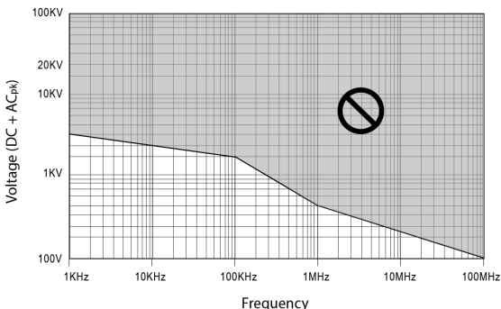
Figure 4: Voltage Derating Curve
