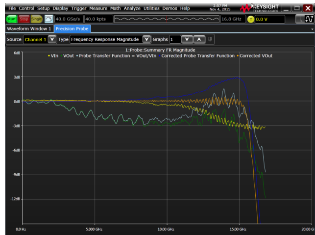
Figure 4. This chart shows the probe/cable's frequency response magnitude and the corrected response.
