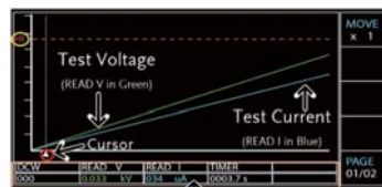
Sweep Function
