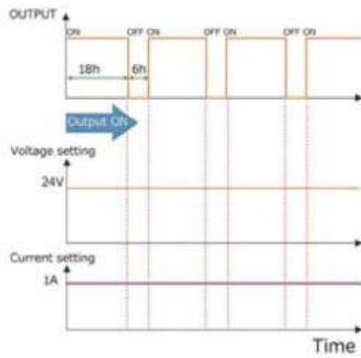
Pattern Setting
