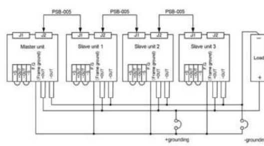
Parallel Connection
