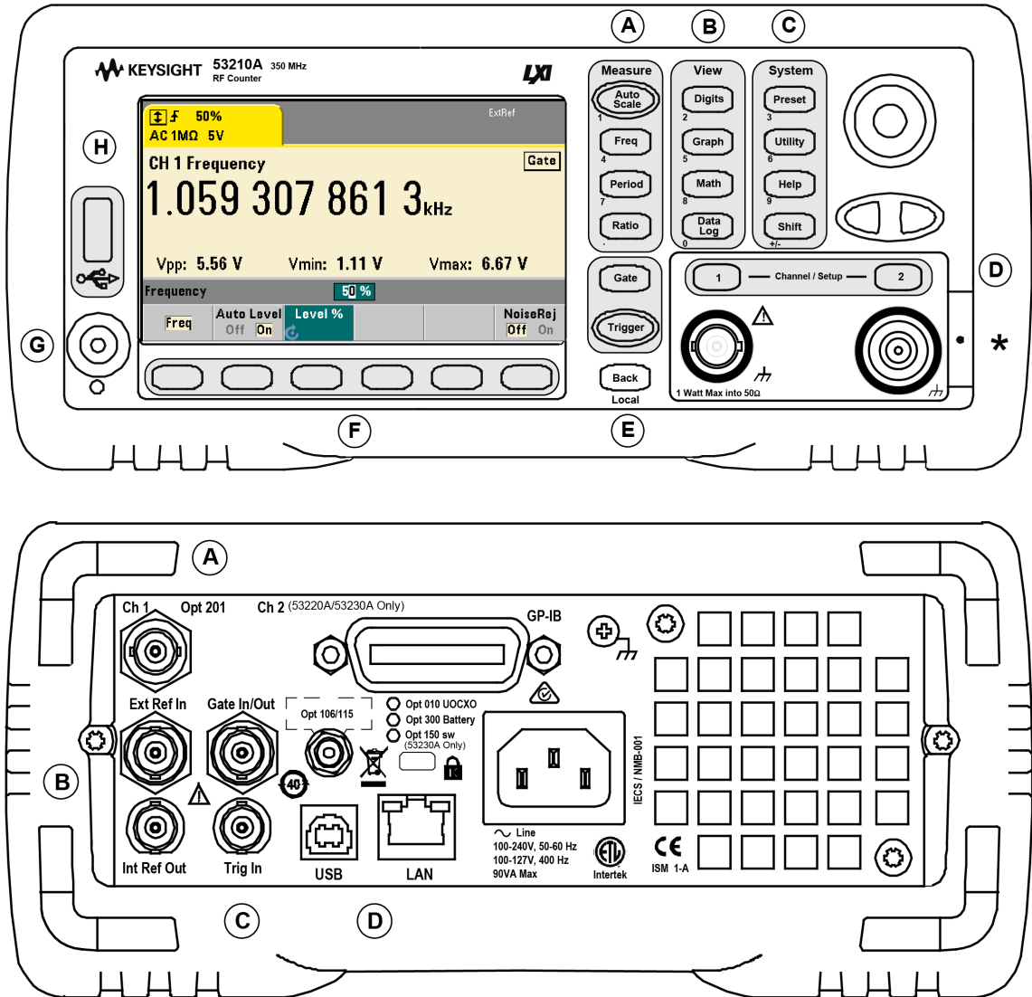
Figure 1-1 The 53210A Universal Frequency Counter/Timer.
