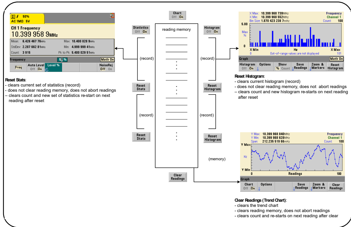
Figure 6-13 Reading Memory and Resetting/Clearing Graphics.
