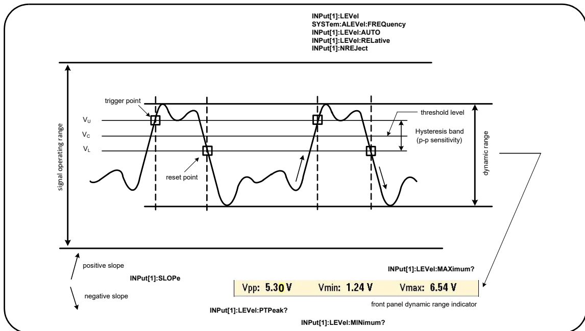
Figure 4-4 Input Signal Threshold Level and Sensitivity.
