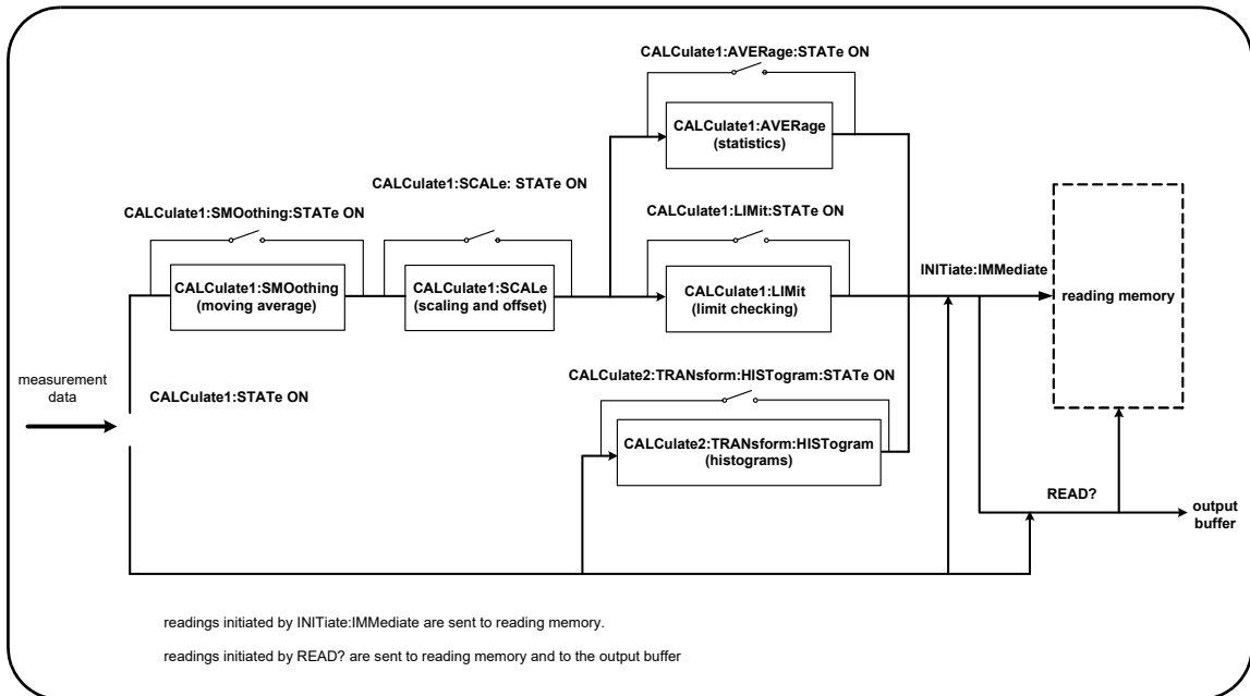
Figure 6-1 Enabling the Math Operations.
