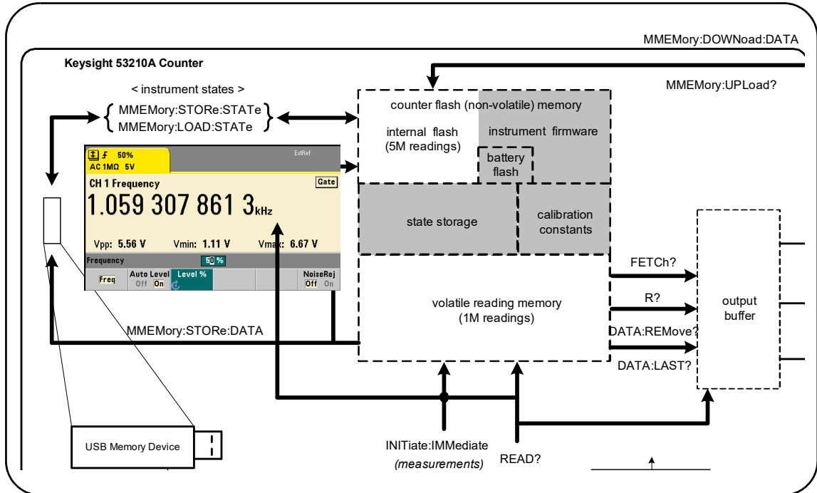
Figure 7-1 Data Flow within the 53210A Counter.
