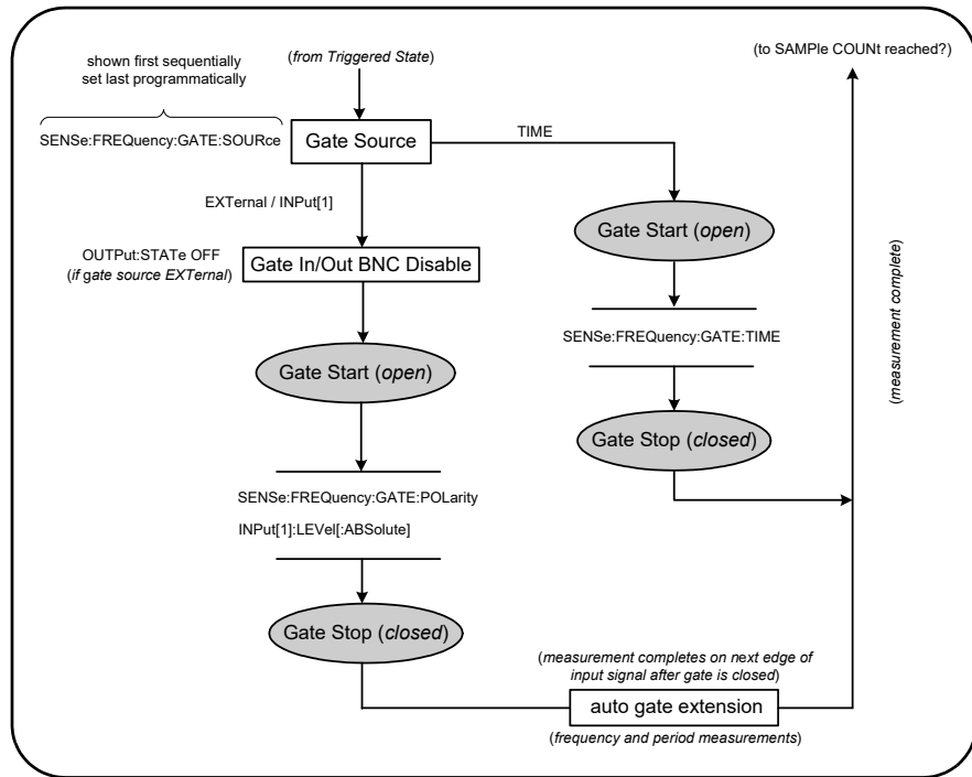
Figure 5-5 Gate Source Sequence.
