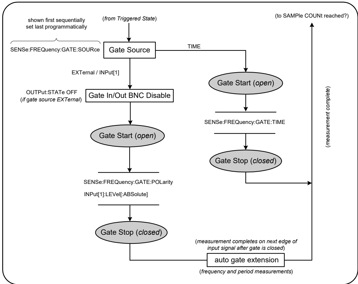
Figure 5-3 Trigger and Gate Cycle - Gating.
