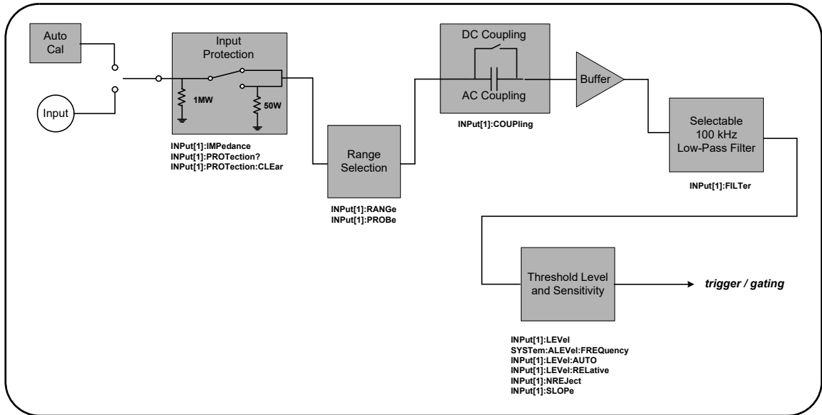
Figure 4-1 53210A Input Signal Conditioning.
