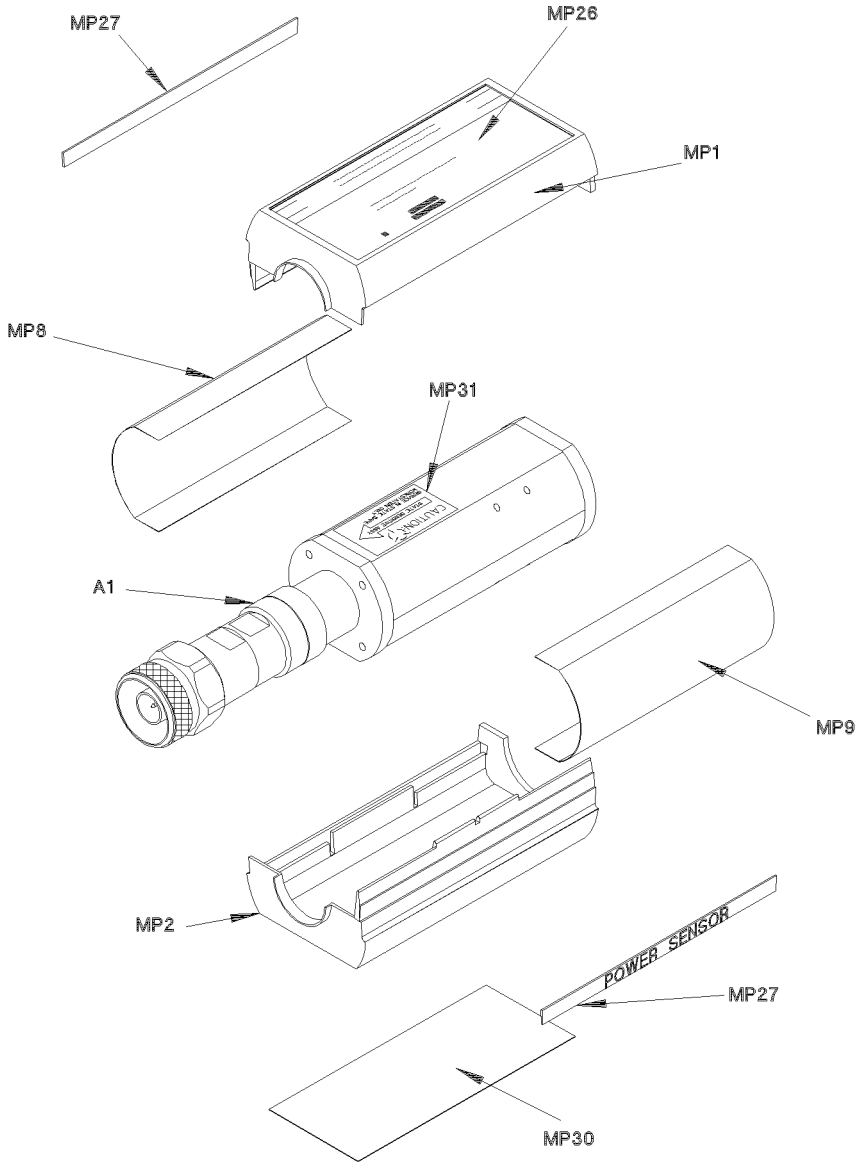
Figure 1-8 Illustrated parts break down
