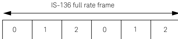
Figure 11-1 A trace display of the active timeslots
