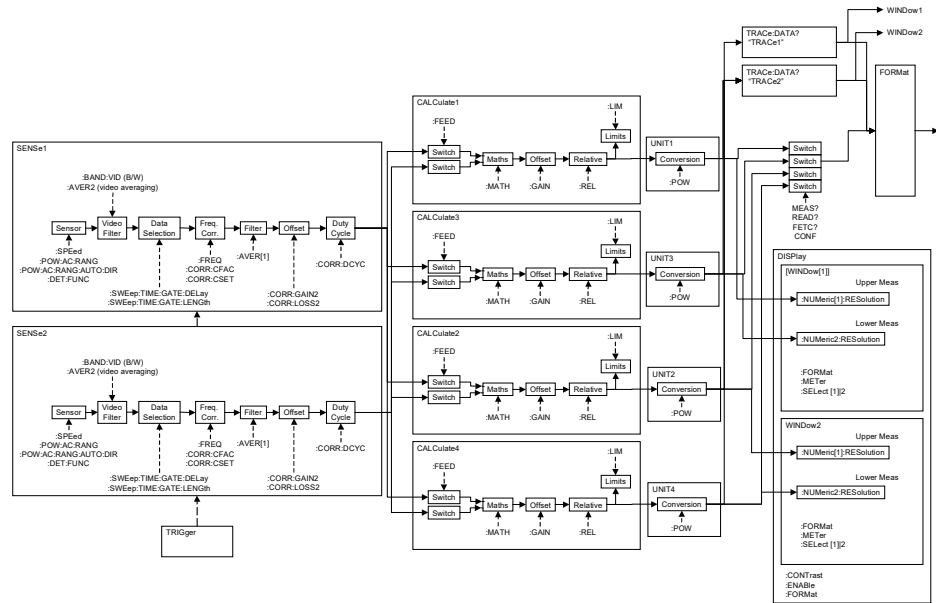
Figure 1-8 How measurements are calculated
