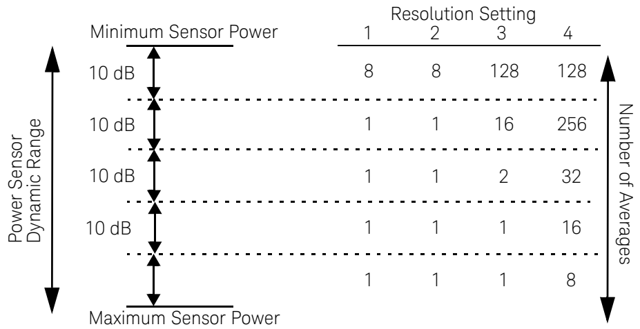
Figure 1-3 Averaged readings
