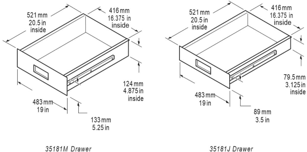
Figure 14. Drawer dimensions
