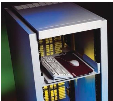
Figure 21. Keyboard when retracted
