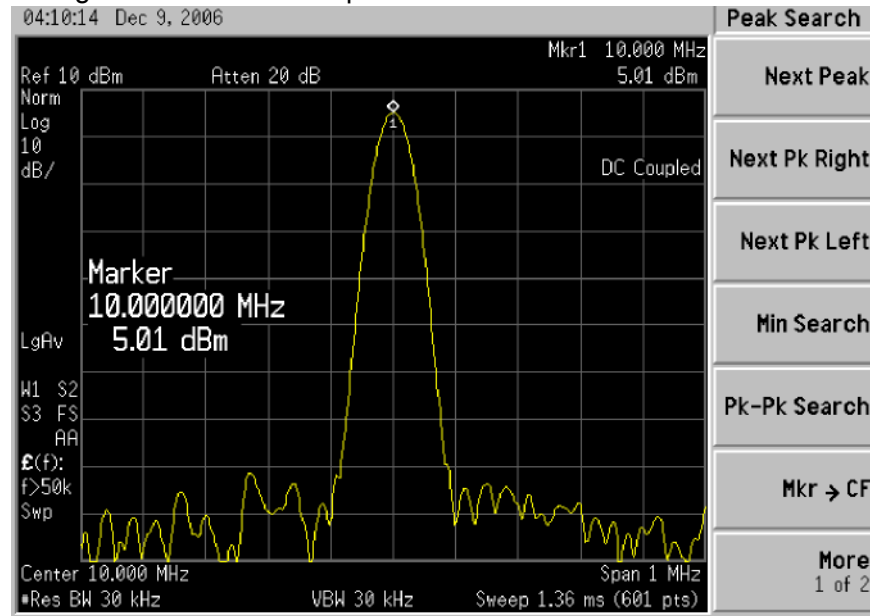
Figure 7-10 A3 Digital I.F. Reference Input
