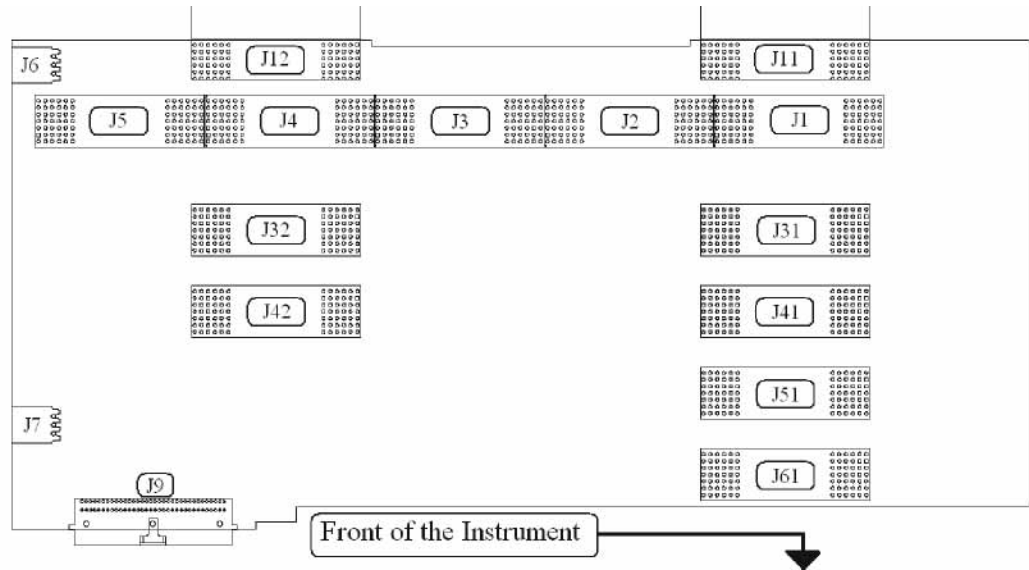
Figure 11-2 Motherboard Connectors
