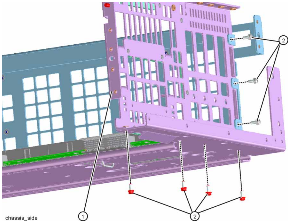
Figure 15-70 Chassis Side Removal
