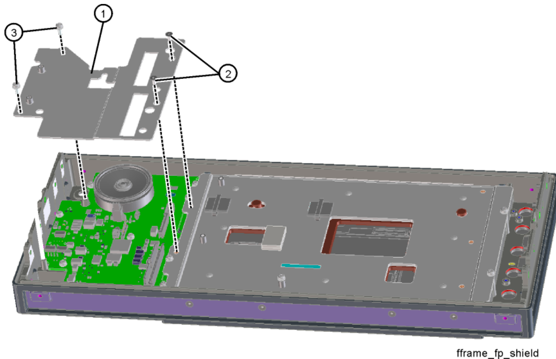
Figure 15-81 Front Panel Control Shield and Board Removal
