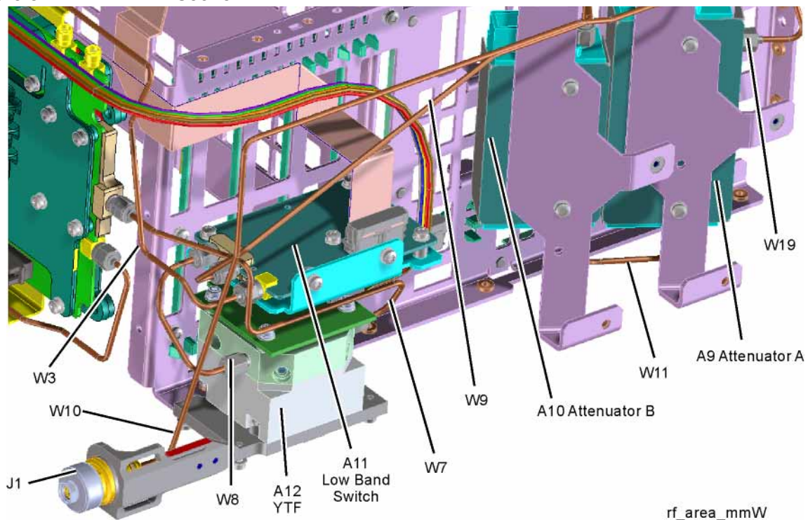
Figure 5-11 RF Section
