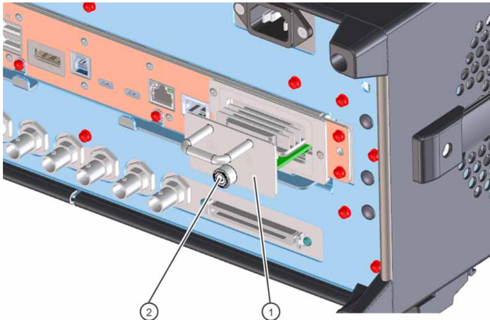
Figure 15-58 SSD Removal
