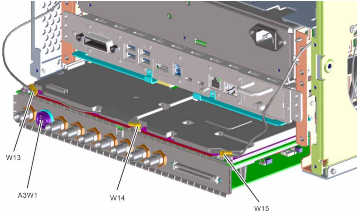
Figure 7-5 A2 Analog I.F. Cables
