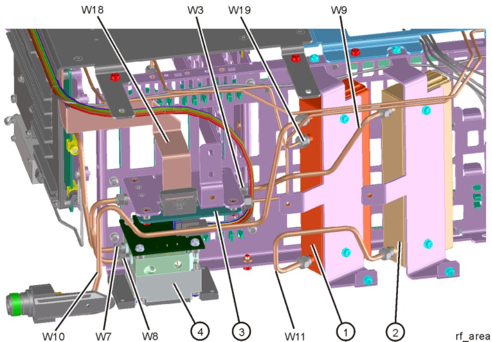
RF Area Components and Cables - Standard RF/Microwave Instruments
