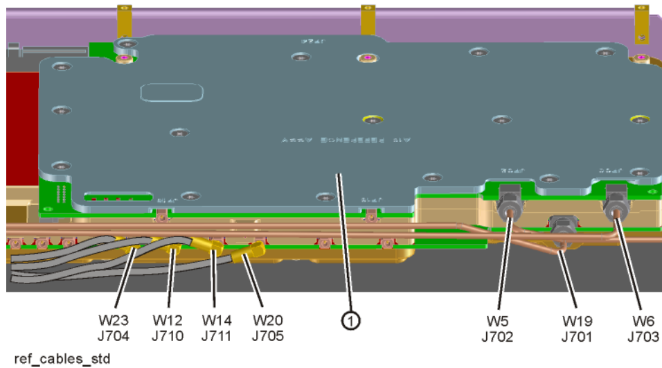
Figure 14-19 Reference Board Cables - without Options B40, MPB, or DP2
