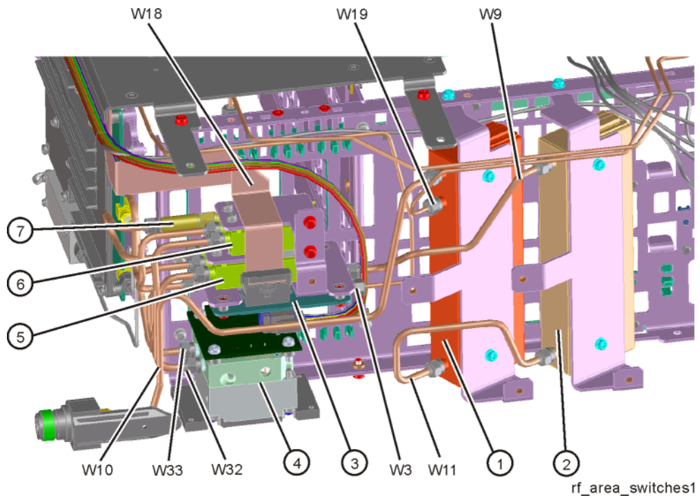
Figure 15-8 RF Area Components and Cables - RF/Microwave Instruments with Options DP2, MPB, B40
