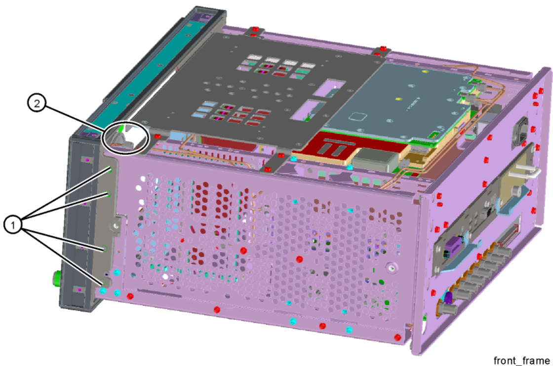
Figure 15-75 Front Frame Assembly Removal
