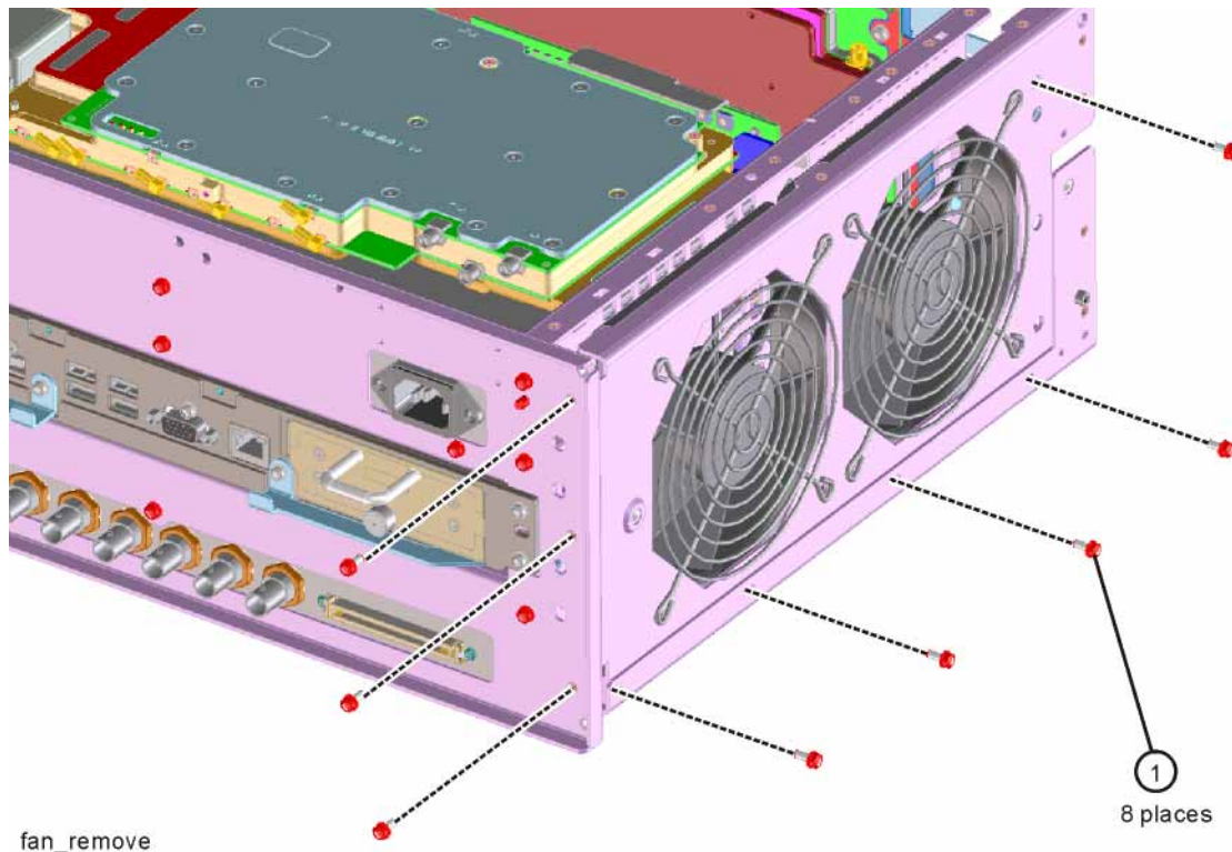
Figure 15-72 Fan Assembly Removal
