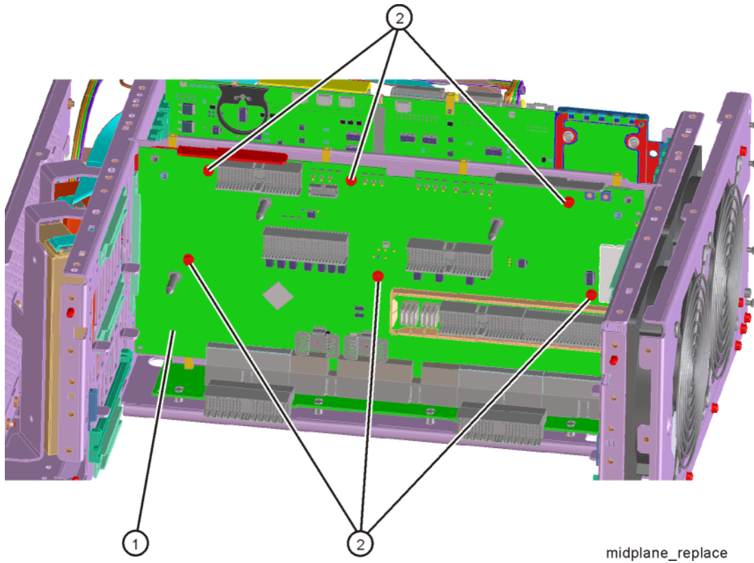
Figure 15-67 Midplane Assembly Removal
