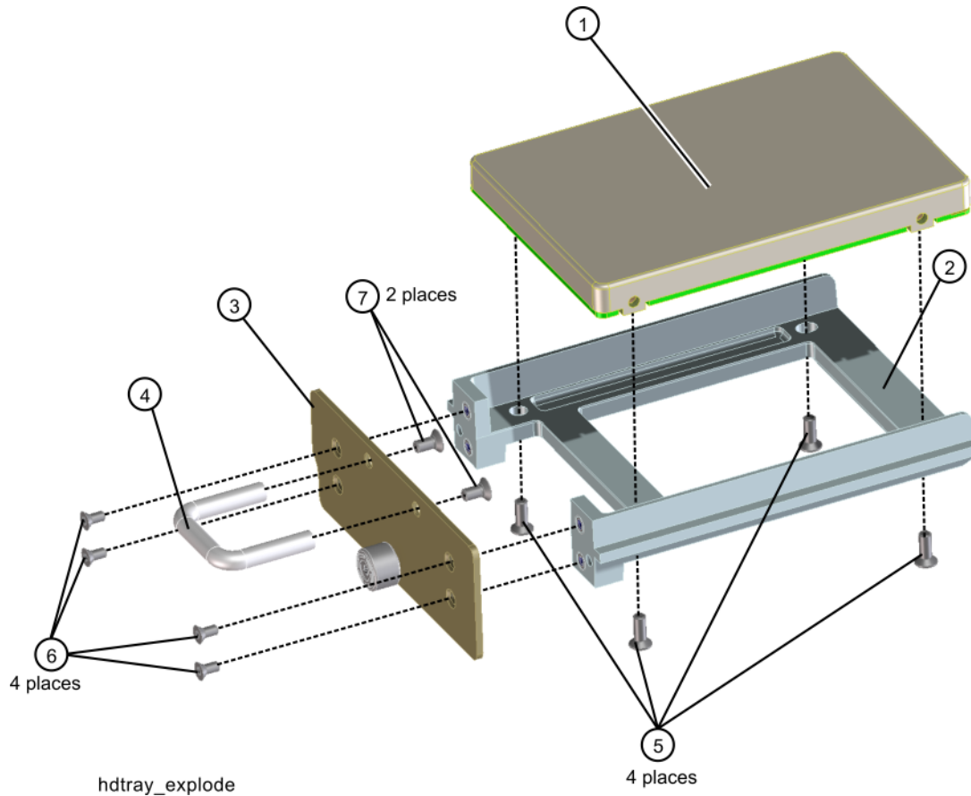
Figure 15-59 Disk Drive Tray Screws
