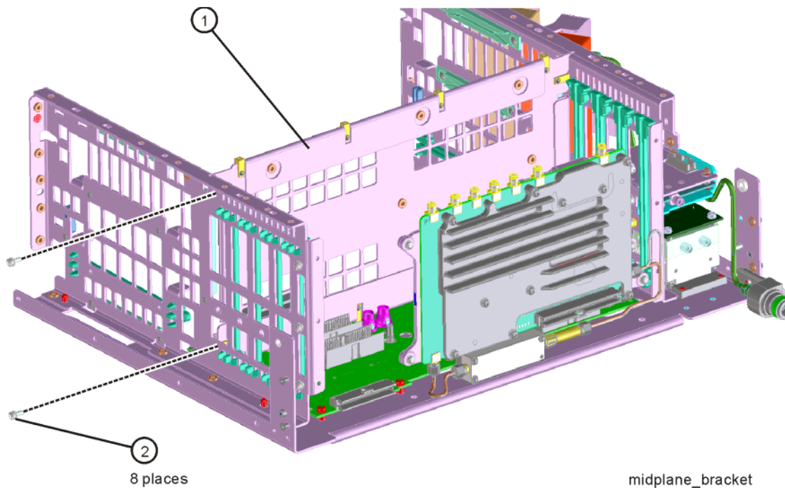
Figure 15-68 Midplane Bracket Removal
