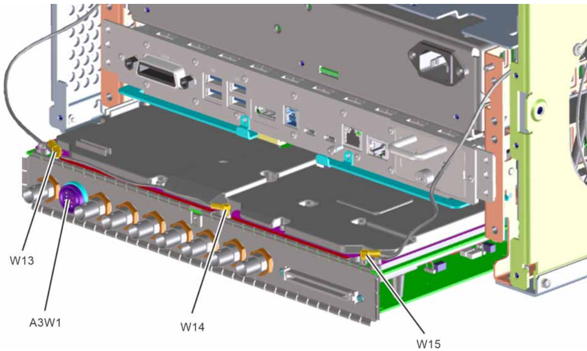
Figure 14-22 AIF/DIF Cables, bottom - Standard Instruments
