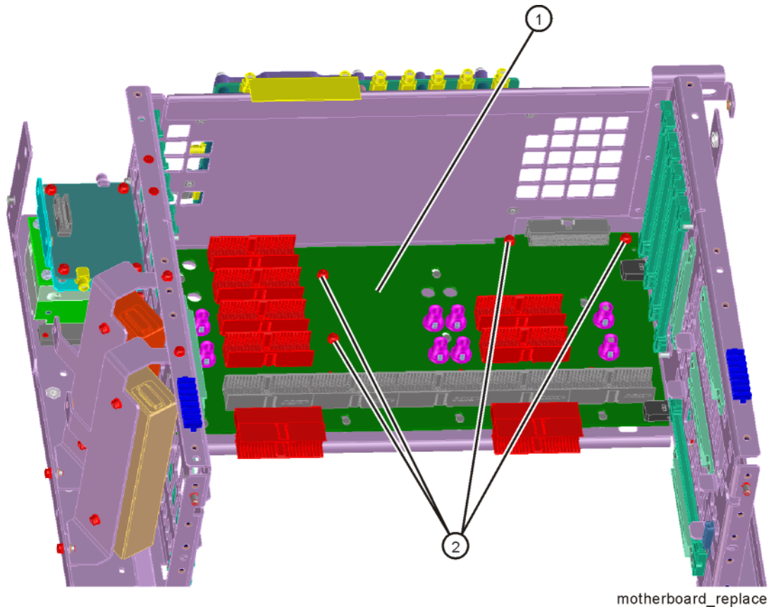
Figure 15-71 Motherboard Assembly Removal
