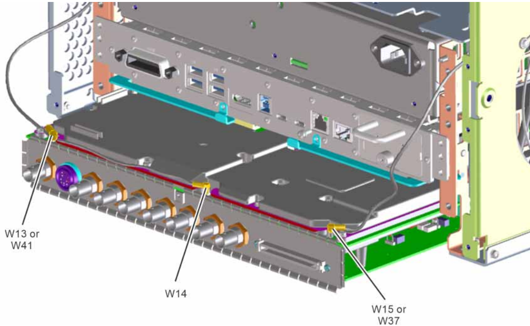
Figure 7-15 A2 Analog IF Cables
