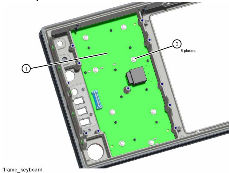
Figure 15-85 Keyboard
