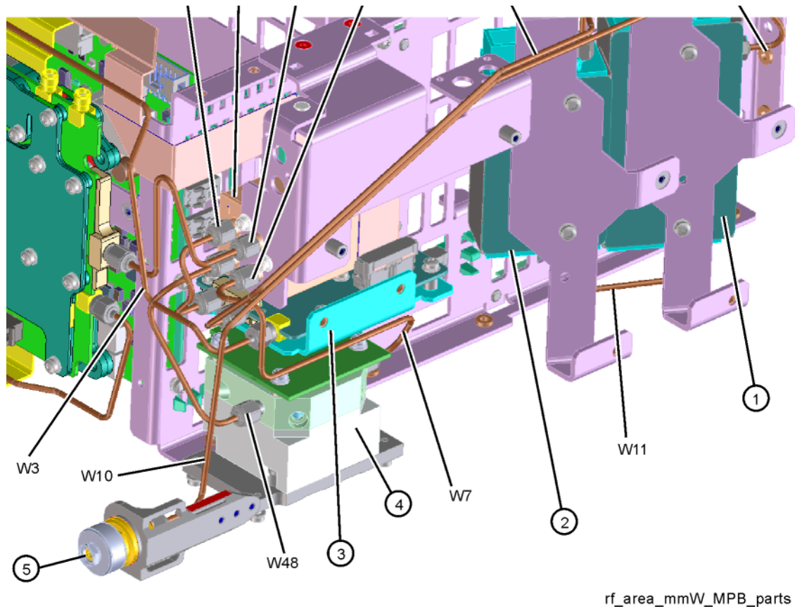
Figure 15-34 RF Area Components and Cables - Option 532, 544 with Option DP2, MPB, B40
