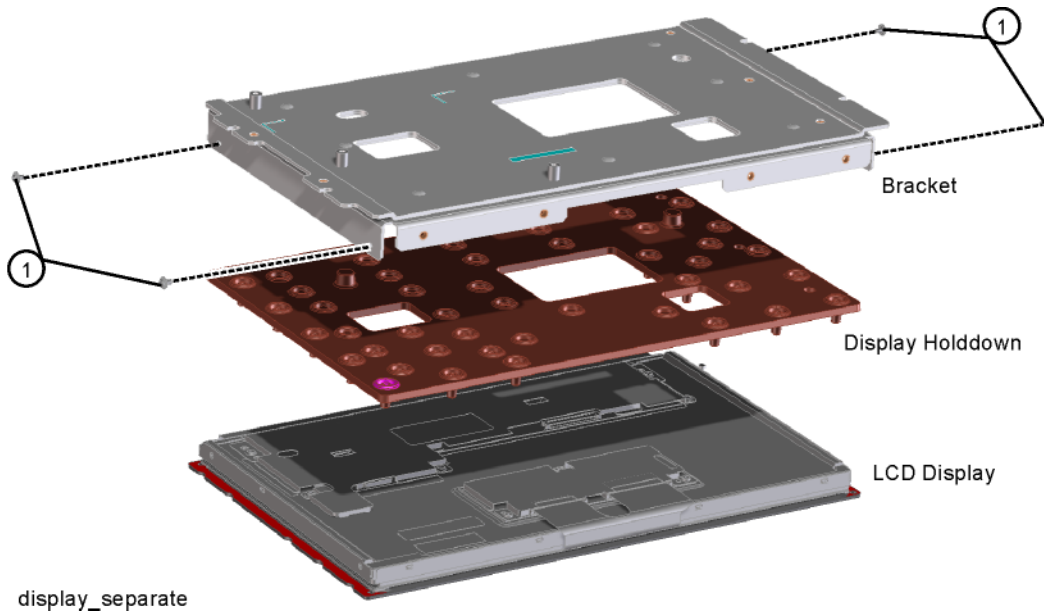
Figure 15-84 Display and Bracket Separation
