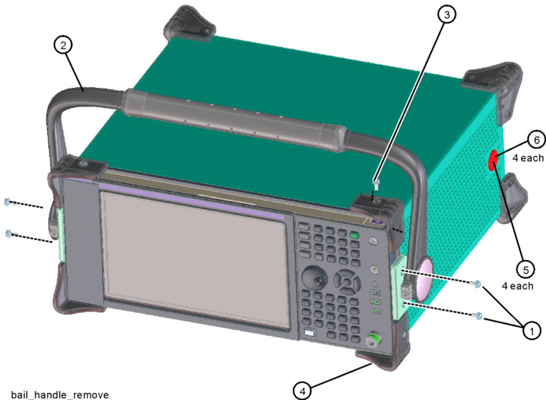
Figure 15-77 Bail Handle and Front Bumpers Removal
