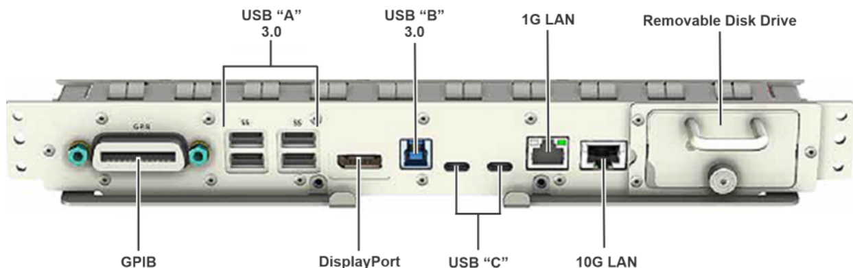
Figure 9-1 A4 Processor Assembly Rear Panel Connectivity (PCB shown)
