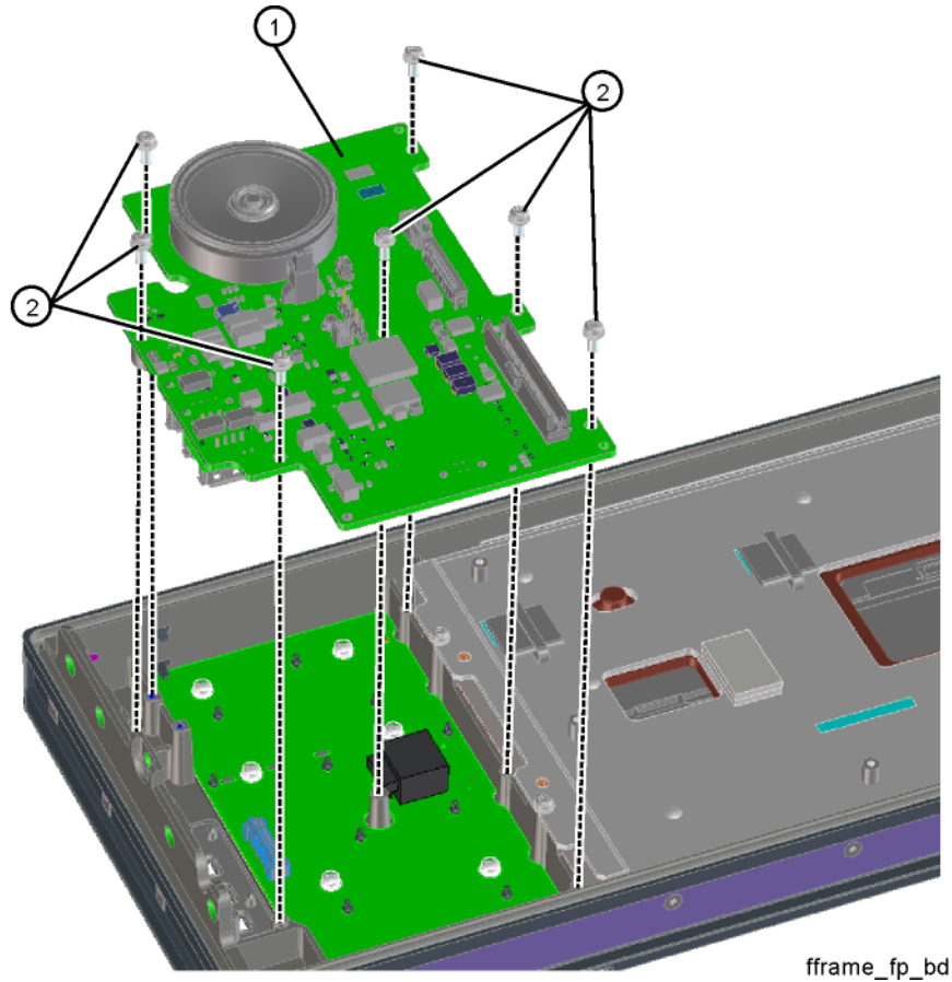
Figure 15-82 Front Panel Control Board
