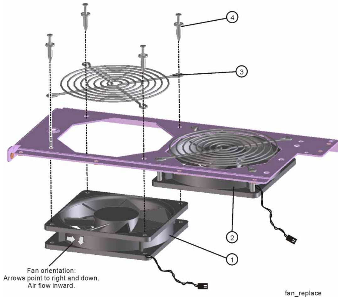
Figure 15-73 Fan Replacement
