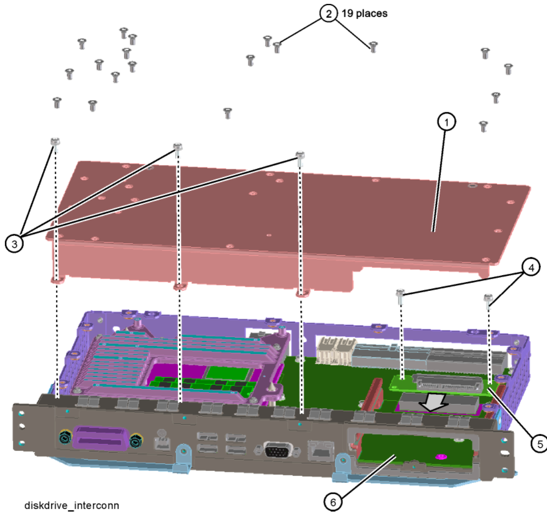
Figure 15-61 A4A1 Disk Drive Interconnect Board Removal
