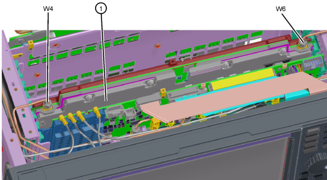
Figure 15-50 L.O. Synthesizer Assembly Removal
