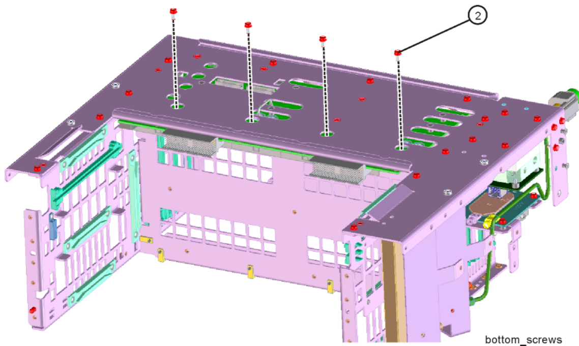
Figure 15-69 Bottom Screws
