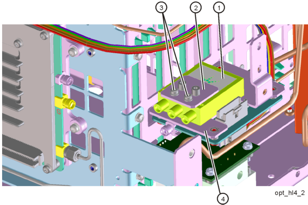
Figure 15-17 Switch 1 Removal
