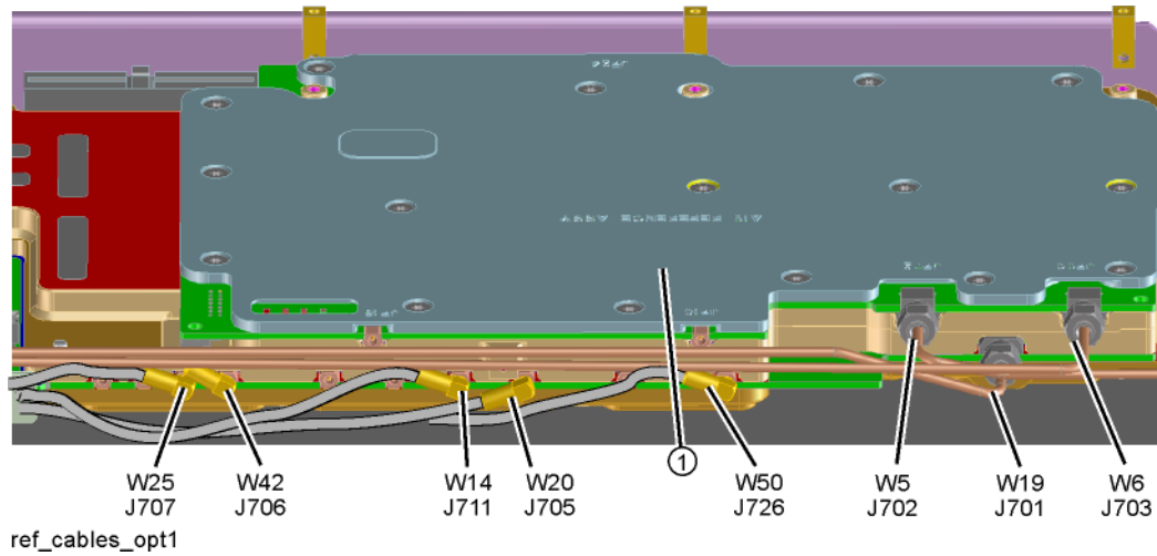
Figure 15-53 Reference Board Cables - with Option B40, MPB, or DP2
