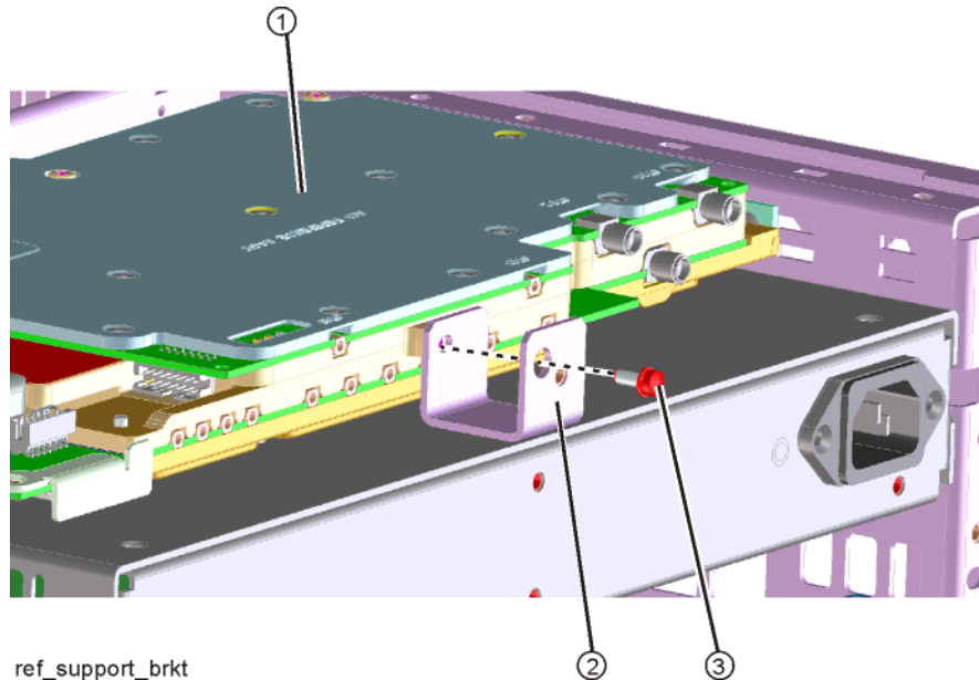
Figure 15-54 Reference Support Bracket Removal
