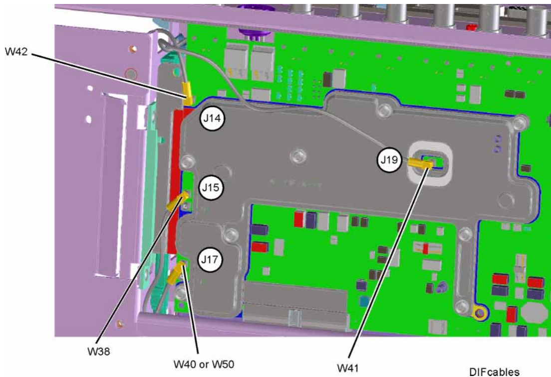
Figure 7-21 A3 Digital IF Cables
