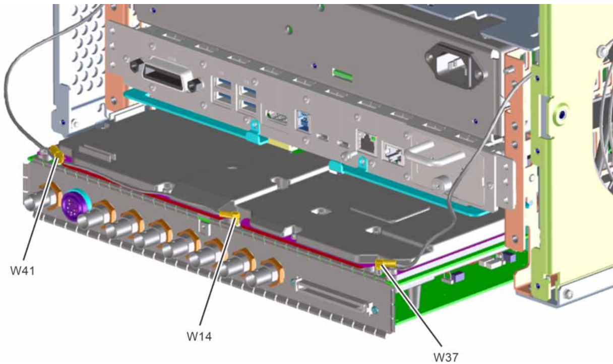
Figure 14-23 AIF/DIF Cables - Options MPB, B40, or DP2
