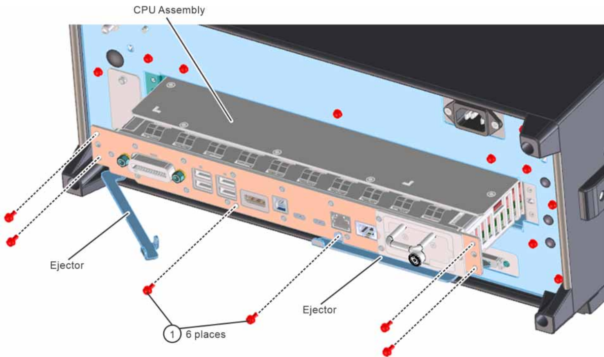
Figure 15-57 CPU Assembly Removal
