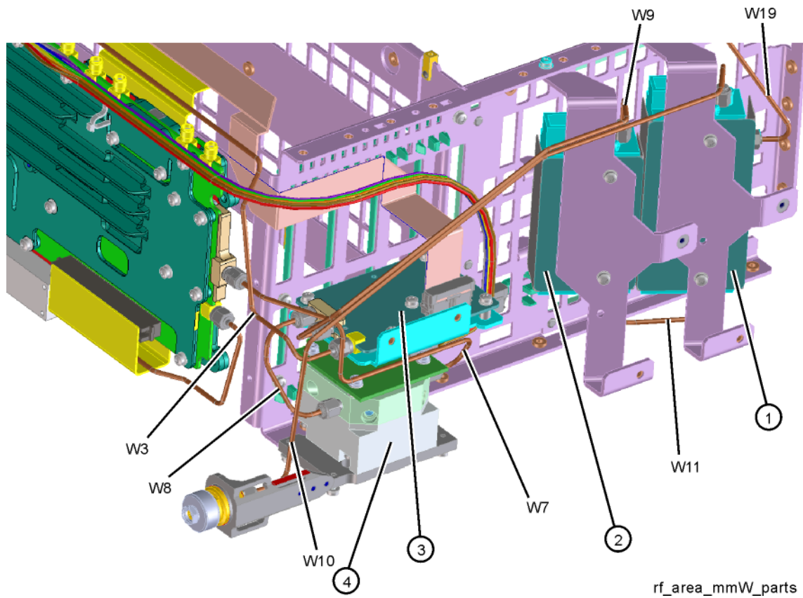
Figure 15-33 RF Area Components and Cables - Option 532, 544
