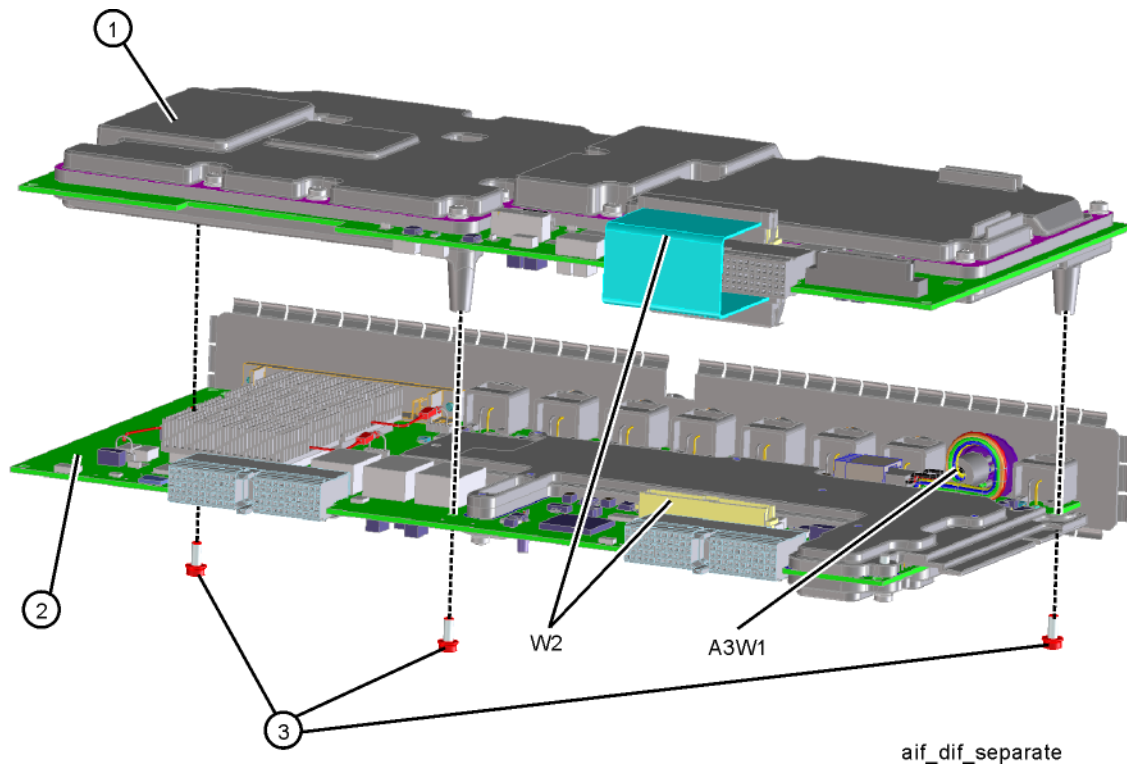
Figure 15-65 AIF/DIF Separation
