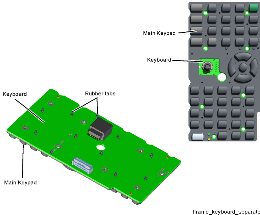
Figure 15-86 Keyboard Keypad Separation
