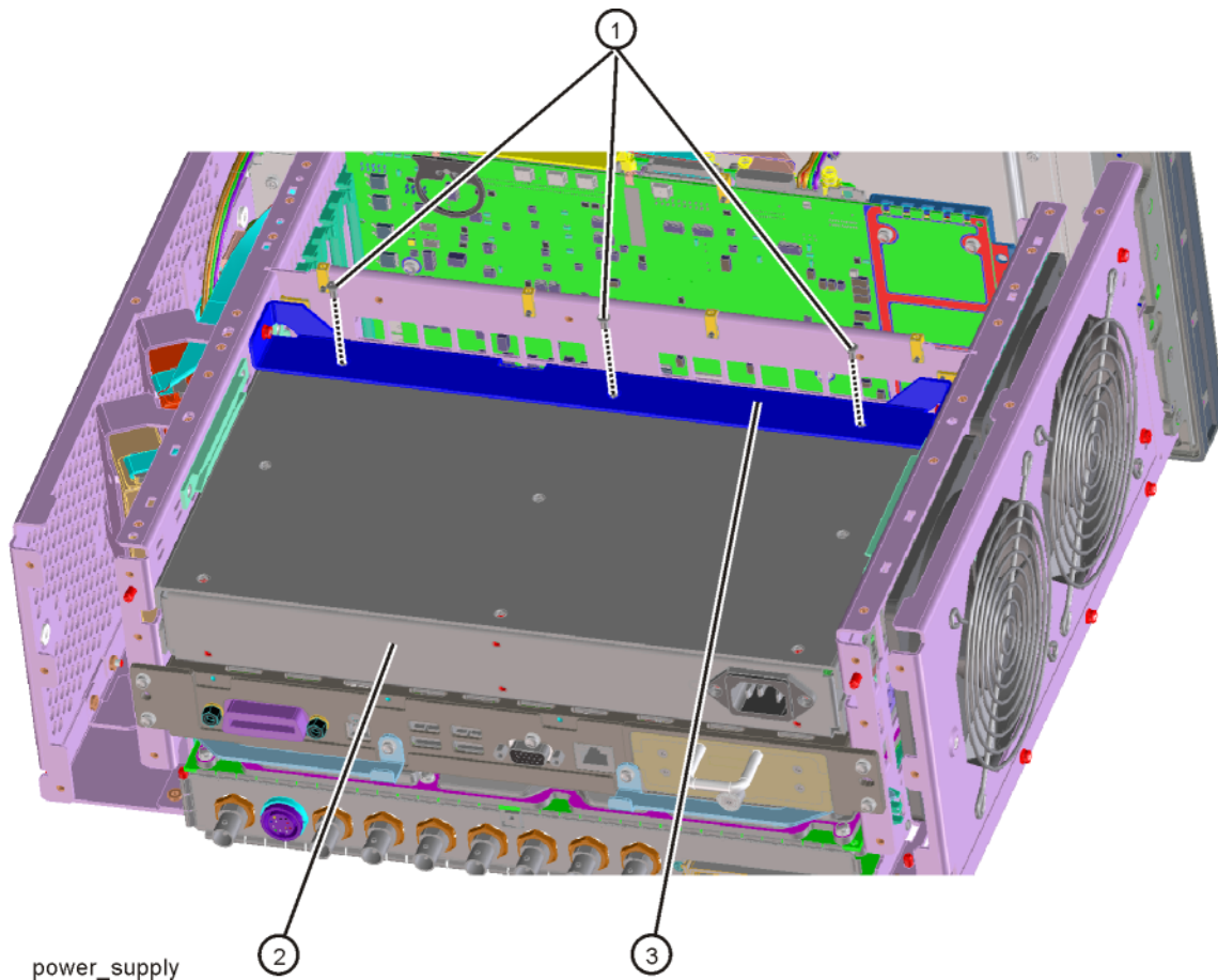
Figure 15-55 Power Supply Assembly Removal
