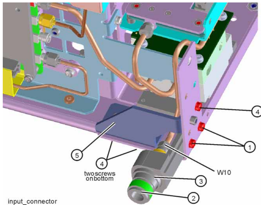
Figure 15-74 Input Connector Assembly Removal
