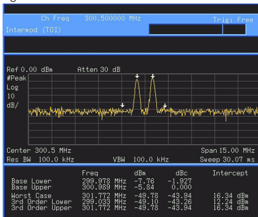
Figure 4-7 TOI Measurement
