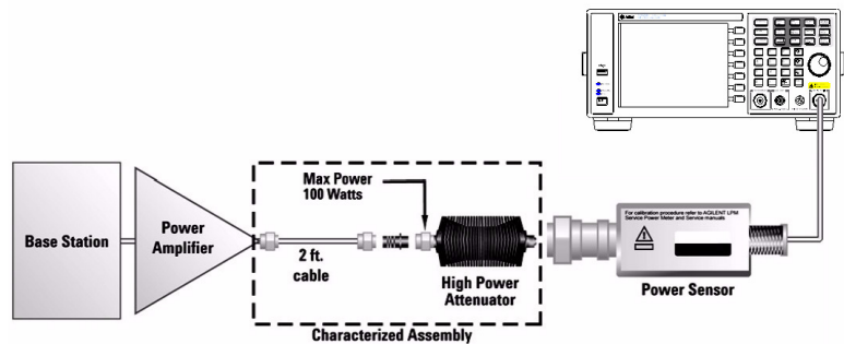
Figure 3-25 Connection with base station
