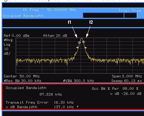
Figure 4-5 Occupied Bandwidth Measurement
