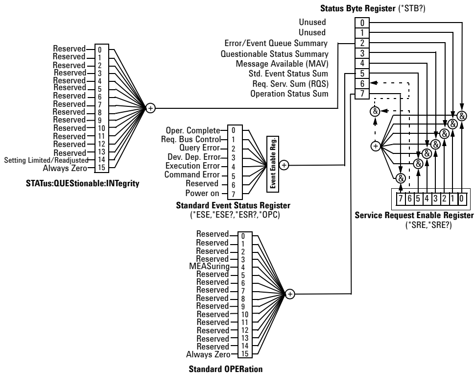
Figure 1 Keysight N9320B Status Register System
