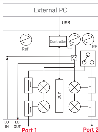
Figure 1. P937XA USB Vector Network Analyzer block diagram
