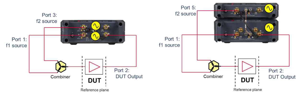
Configuration using a 4-port P502xA (left), 6-port configuration using 2-port P500xA and 4-port P502xA (right).
