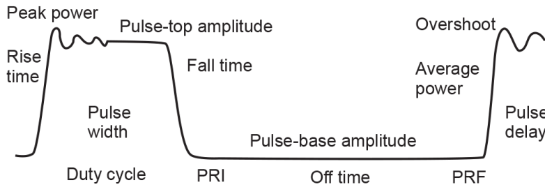
Figure 1-1. Typical envelope of pulsed system with overshoot and pulse ringing, shown with 13 pulse parameters which the Keysight 8990A characterized for time and amplitude.
