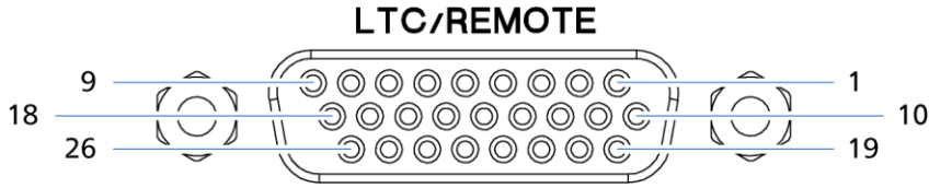
Figure 6-1 | LTC/REMOTE
