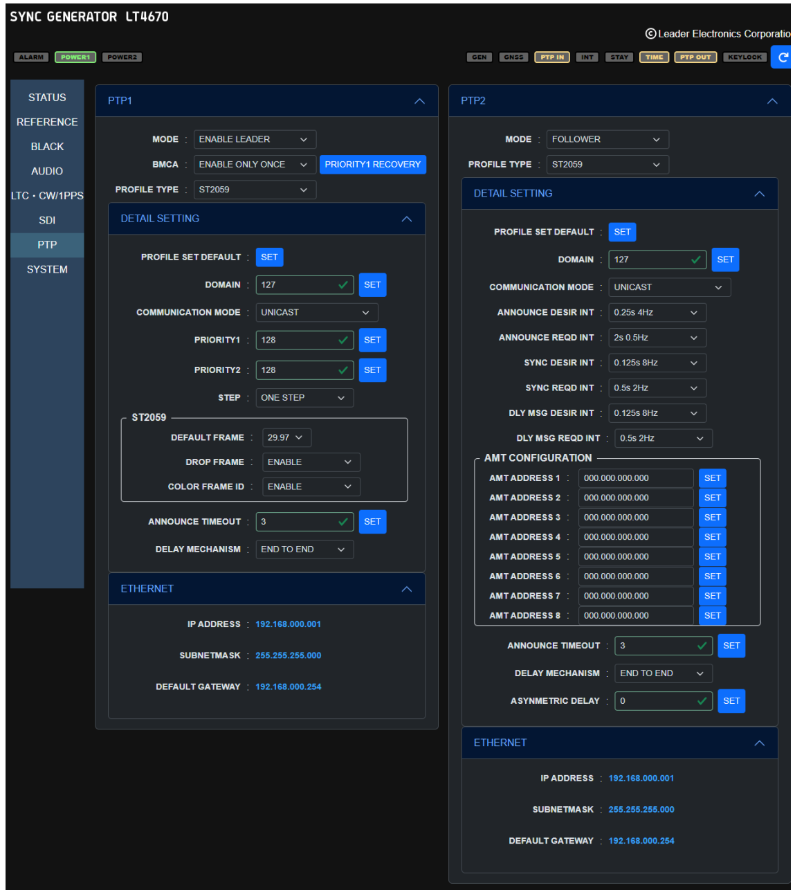
Figure 17-14 | PTP screen
