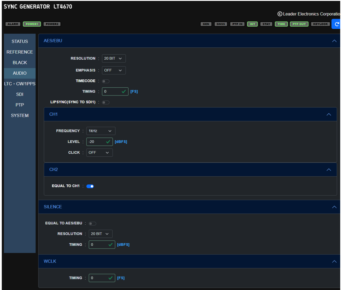
Figure 17-11 | AUDIO screen
