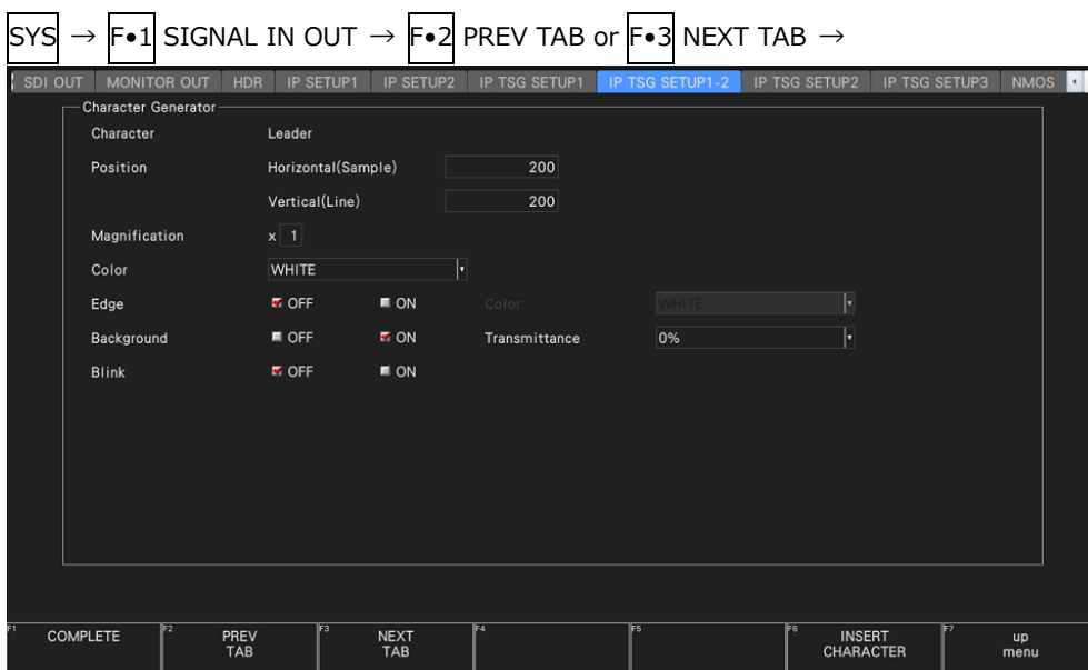
Figure 7-18 IP TSG SETUP1-2 tab
