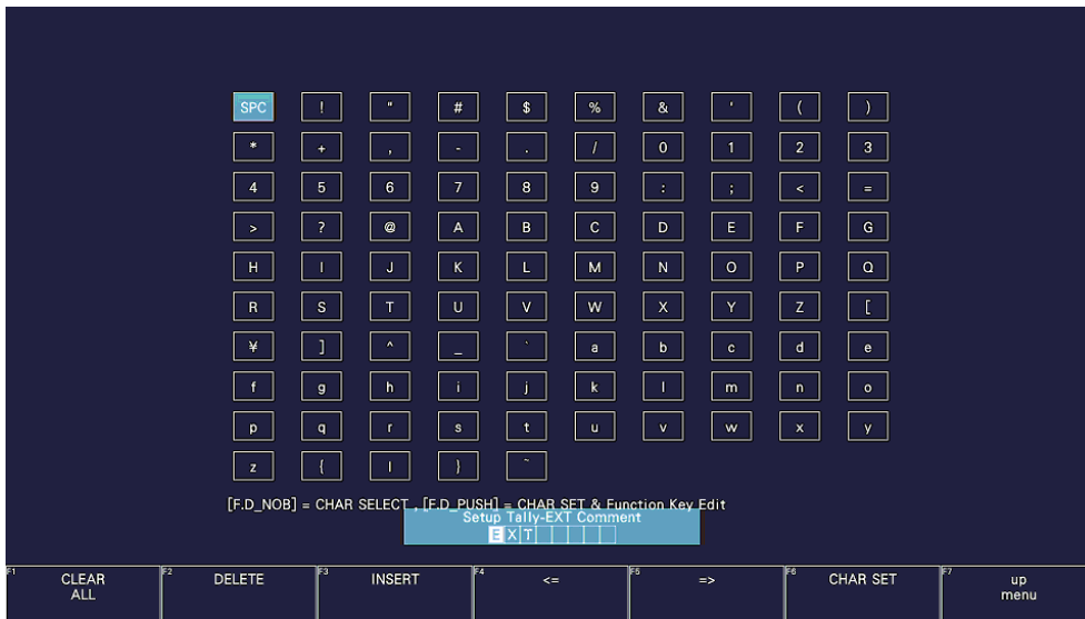
Figure 7-42 Comment input screen
