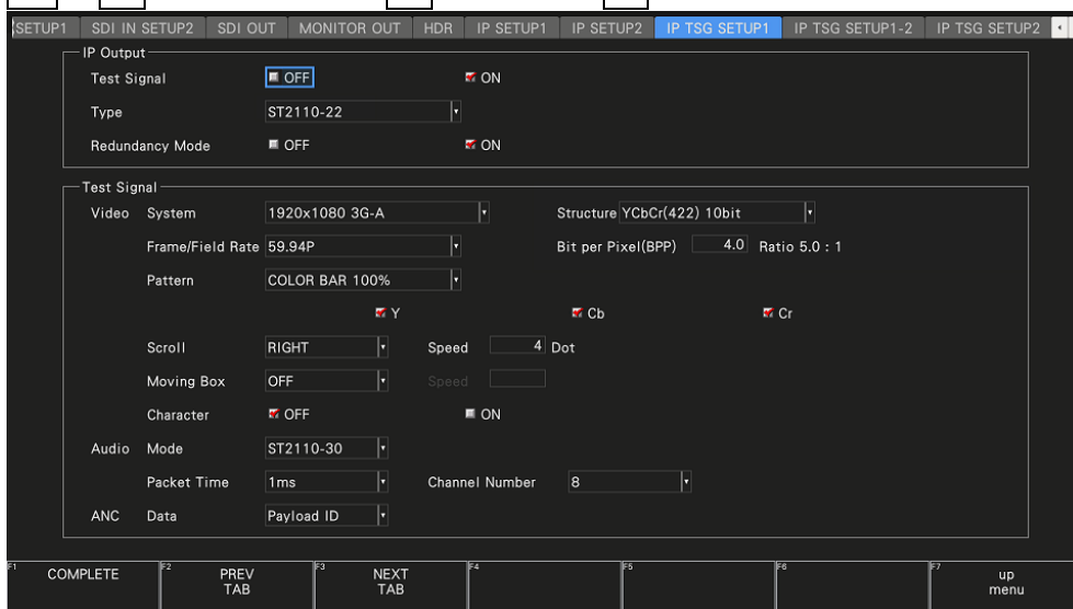
Figure 7-16 IP TSG SETUP1 tab
