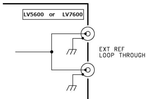
Figure 5-4 Loop-through
