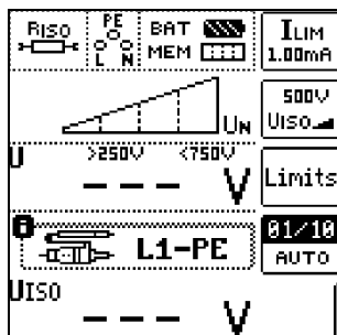
Insulation Measurement
