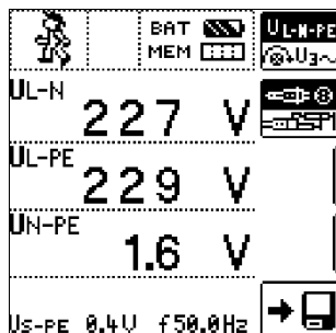
Voltage Measurement
