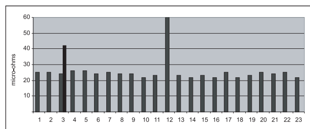
Figure 7 Intercell connection resistance bar graph
