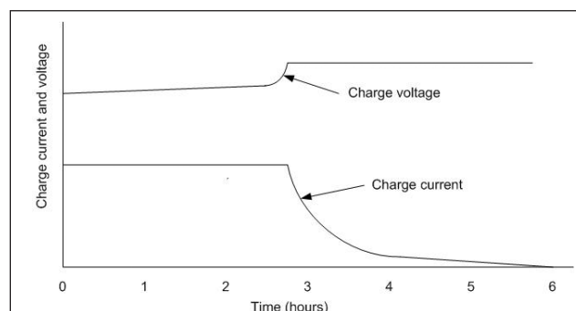
Figure 8 Constant-voltage Constant-current charge characteristics
