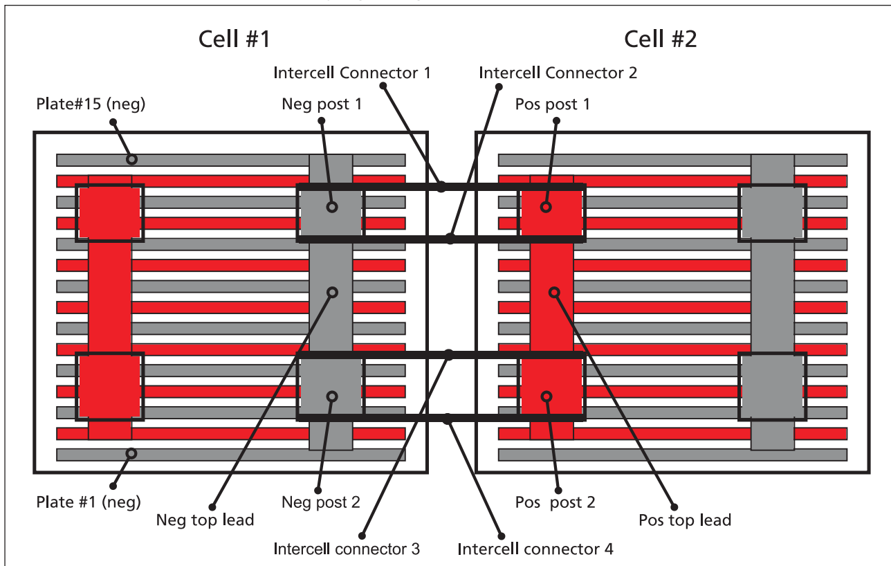
Figure 1 Battery construction diagram
