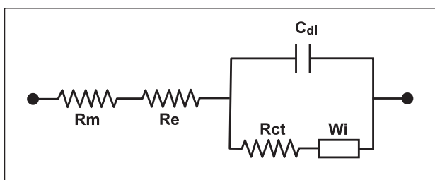
Figure 6 Randles equivalent circuit
