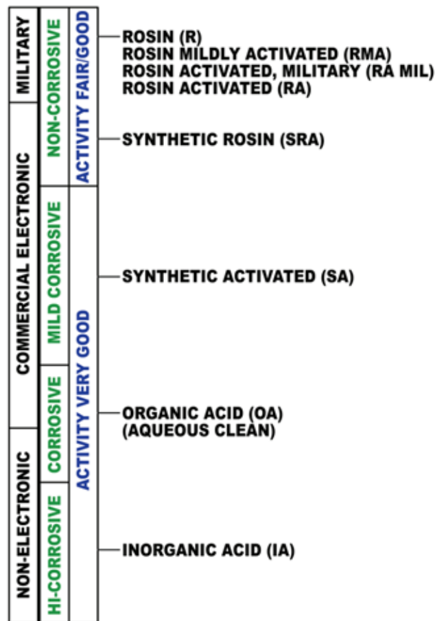
Figure 4: Flux Types
