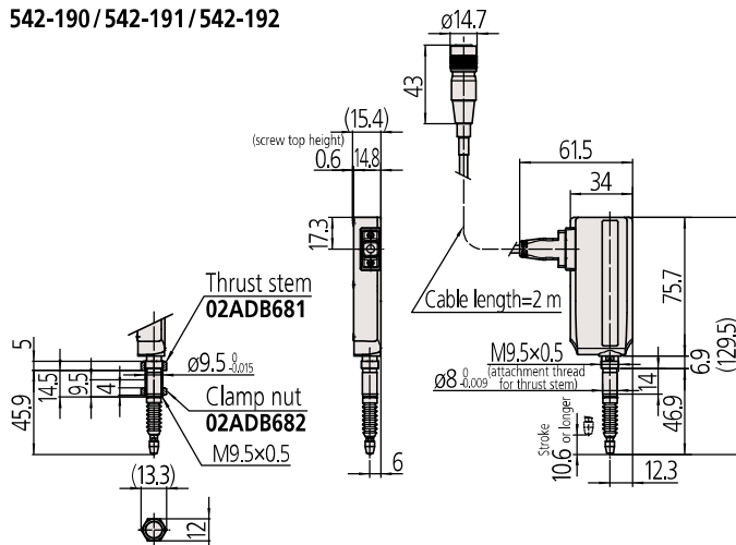
Dimensions with an optional thrust stem installed
