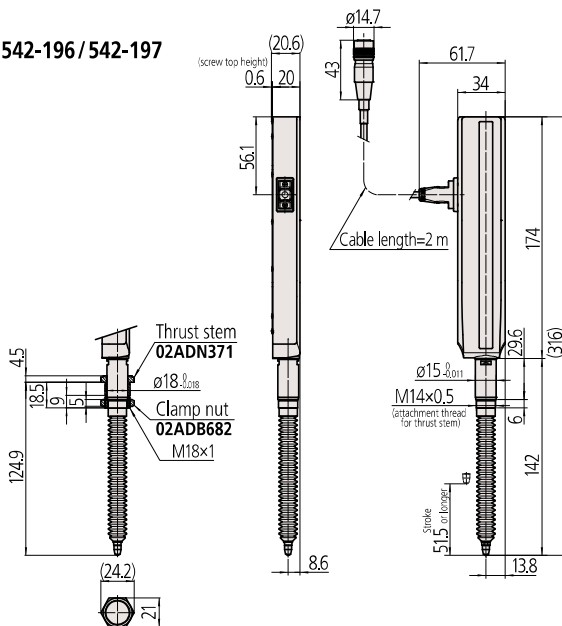
Dimensions with an optional thrust stem installed
