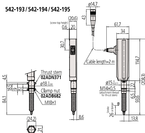
Dimensions with an optional thrust stem installed
