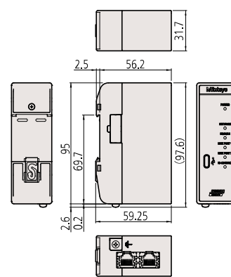
Interface unit PROFINET
