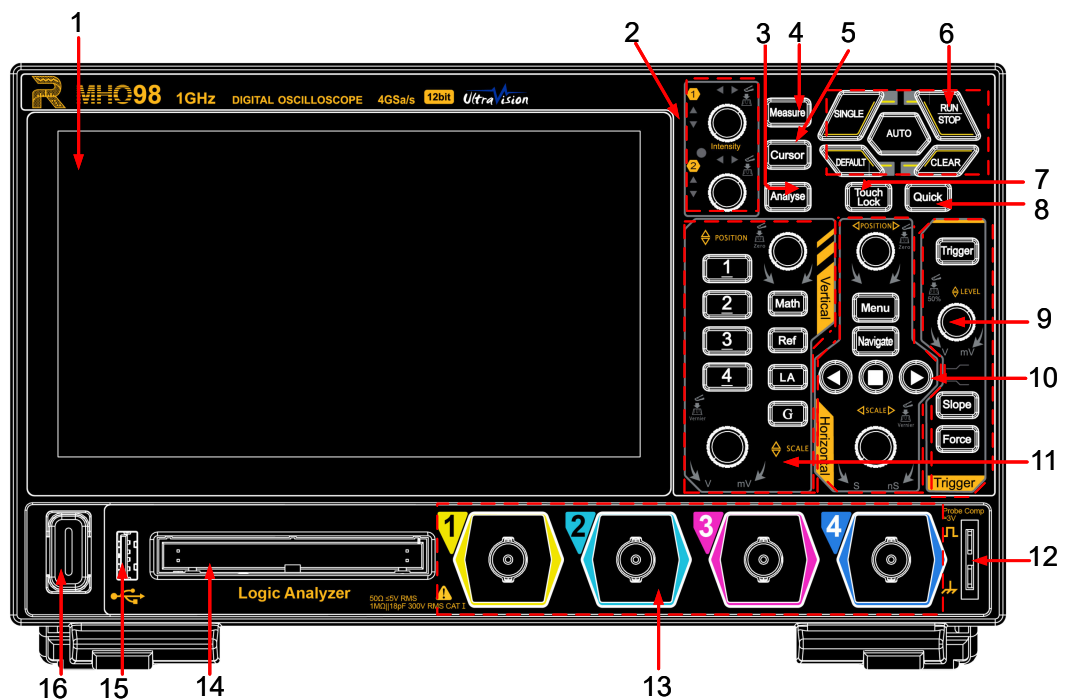
Figure 4.3 Front Panel
