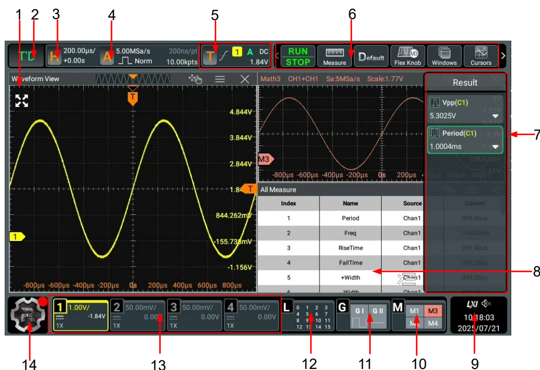
Figure 4.5 User Interface
