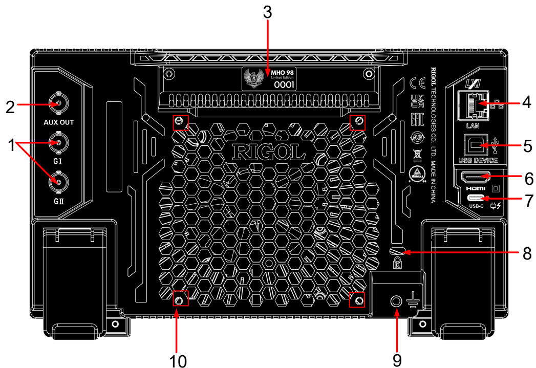
Figure 4.4 Rear Panel
