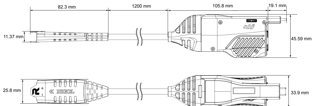
Figure 4.1 Probe Size
