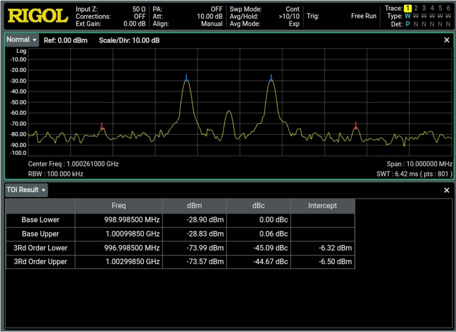
Figure 5.6 TOI Distortion Measurement Interface
