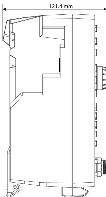
Figure 4.2 Side view (mm)
