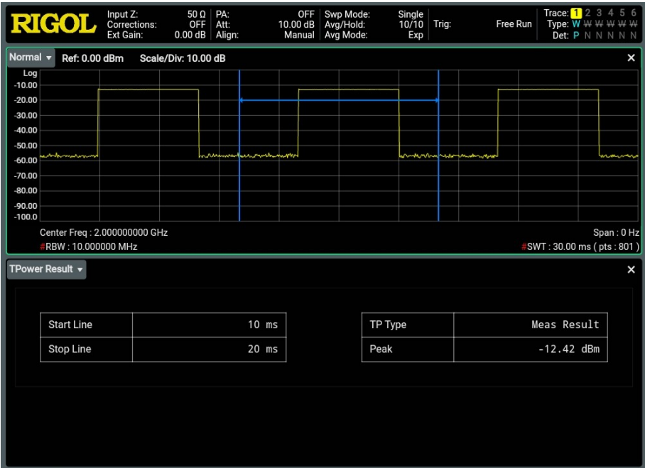
Figure 5.9 T-Power Measurement Interface
