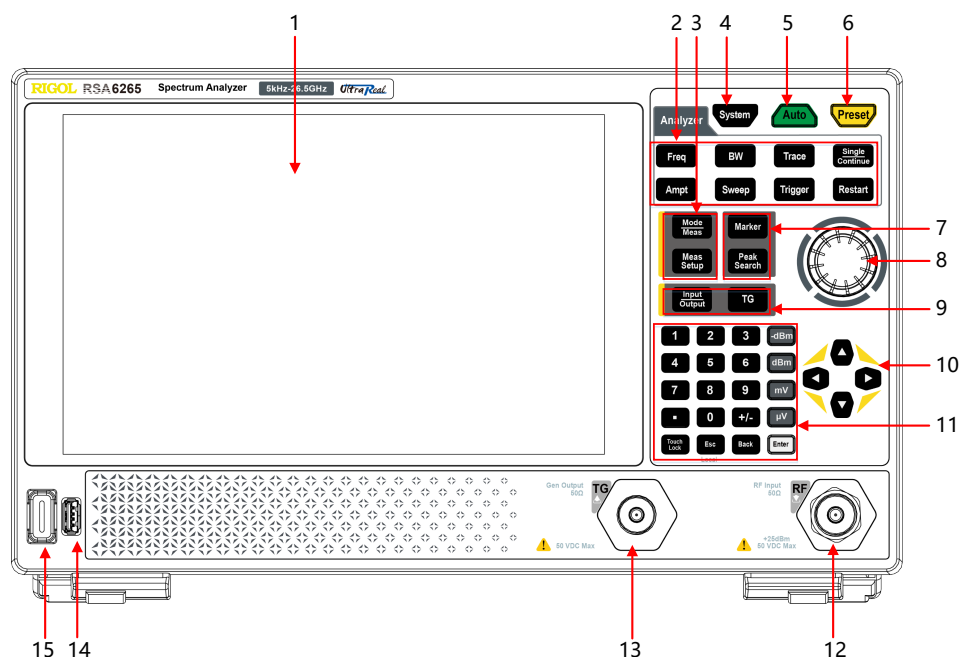
Figure 4.4 Front Panel
