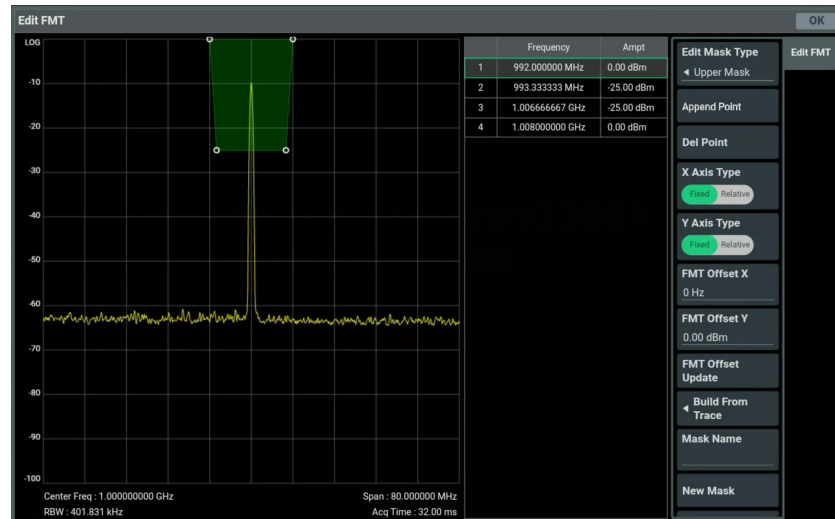
Figure 6.8 FMT Editing Interface
