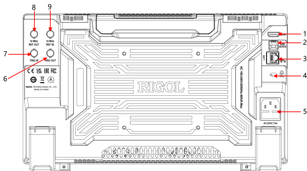
Figure 4.8 Rear Panel
