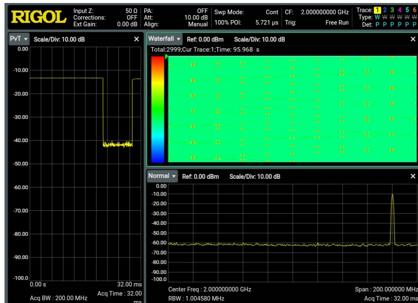
Figure 6.7 PvT/Normal/Waterfall Plot View
