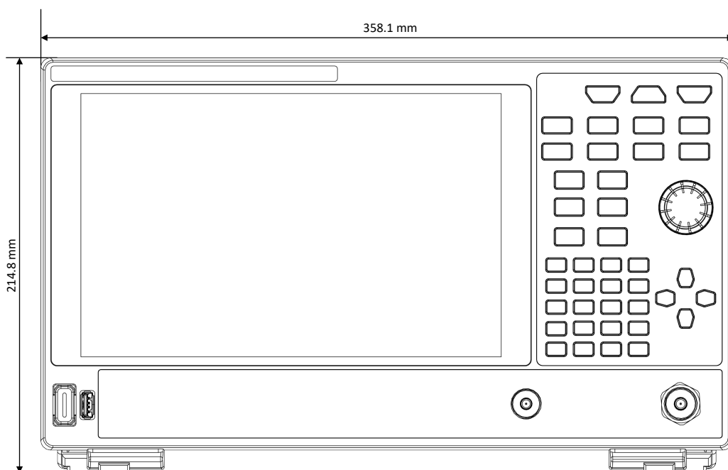
Figure 4.1 Front view (mm)
