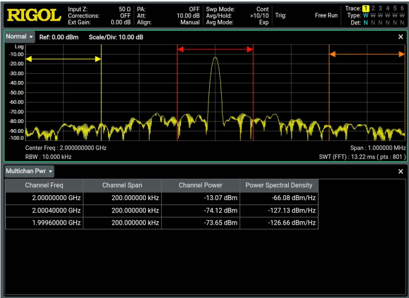
Figure 5.5 Channel Power Measurement Interface
