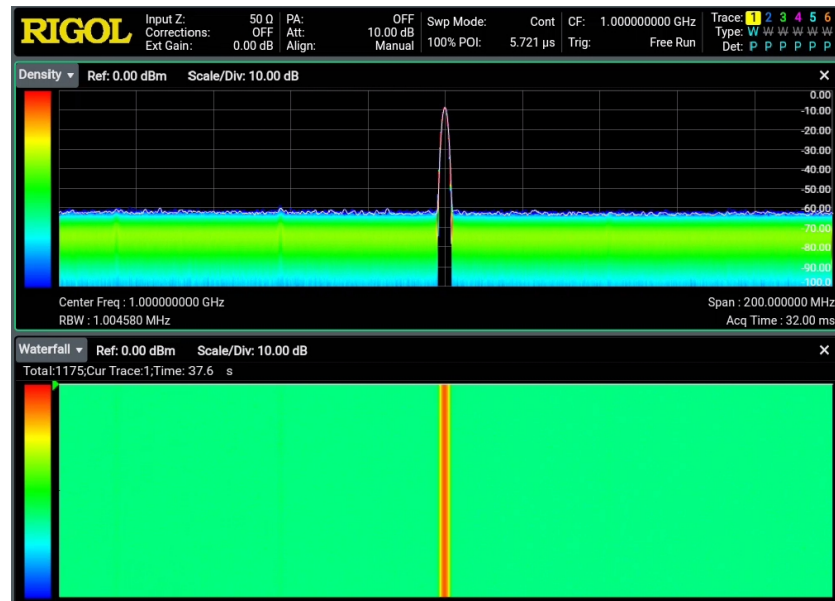
Figure 6.4 Density/Waterfall Plot View
