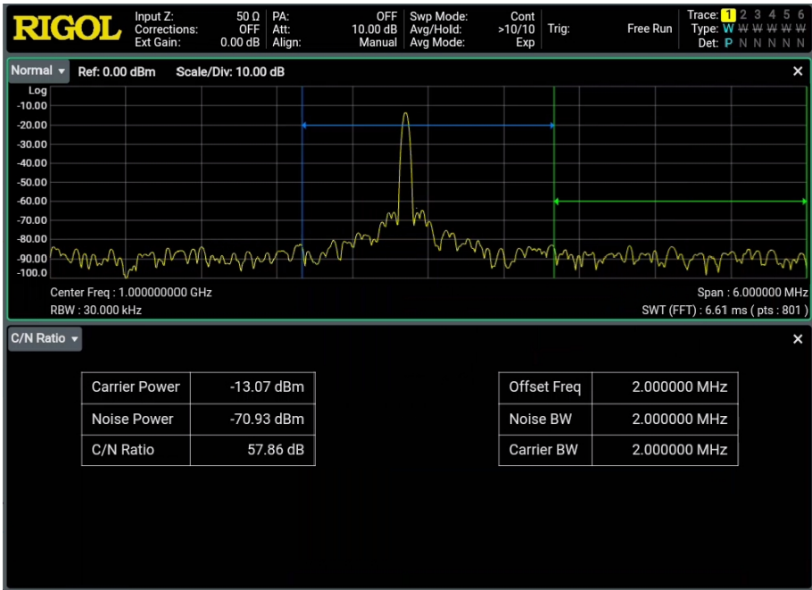
Figure 5.4 C/N Ratio Measurement Interface
