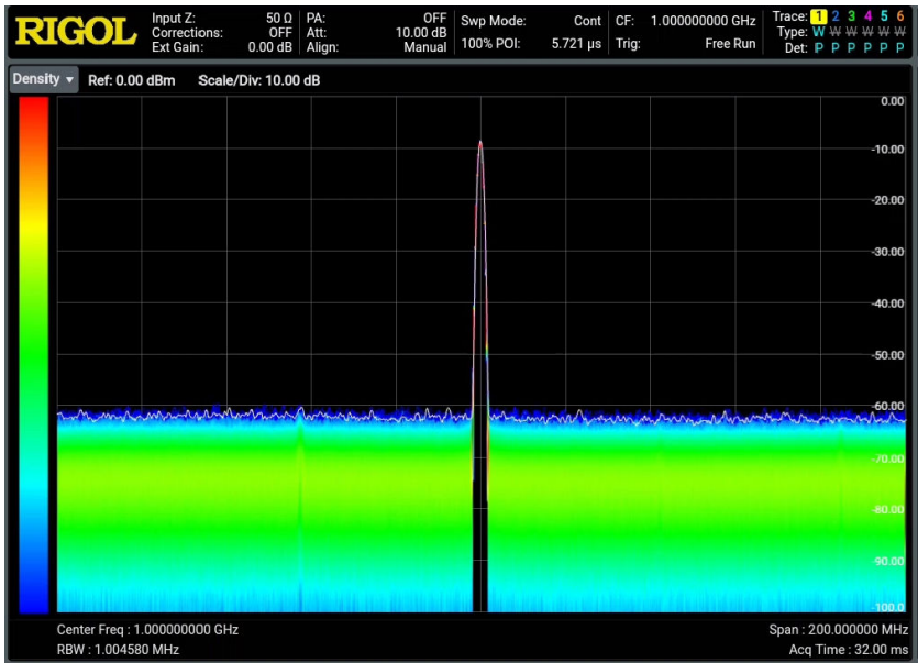
Figure 6.3 Density Display View
