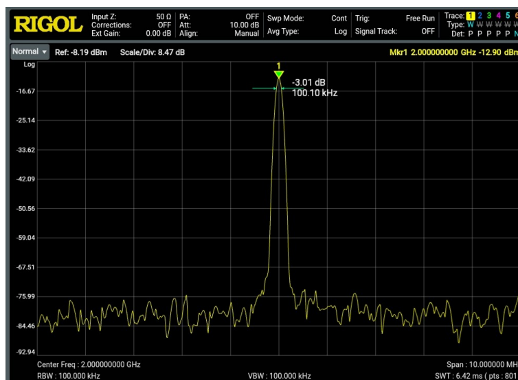
Figure 5.12 N dB Bandwidth Measurement
