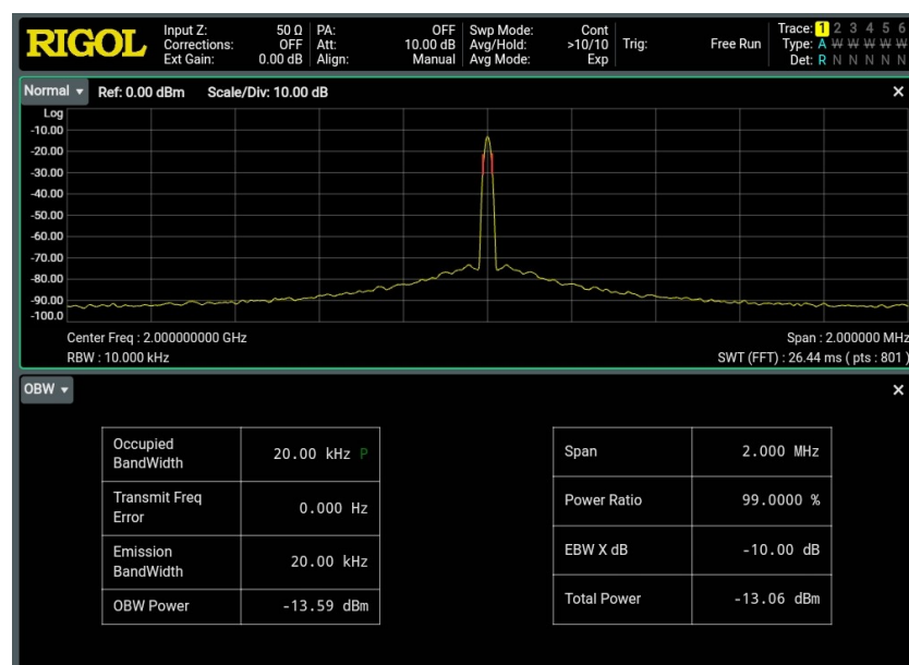
Figure 5.8 OBW Measurement Interface
