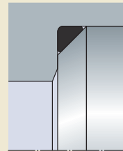
Triangular groove
