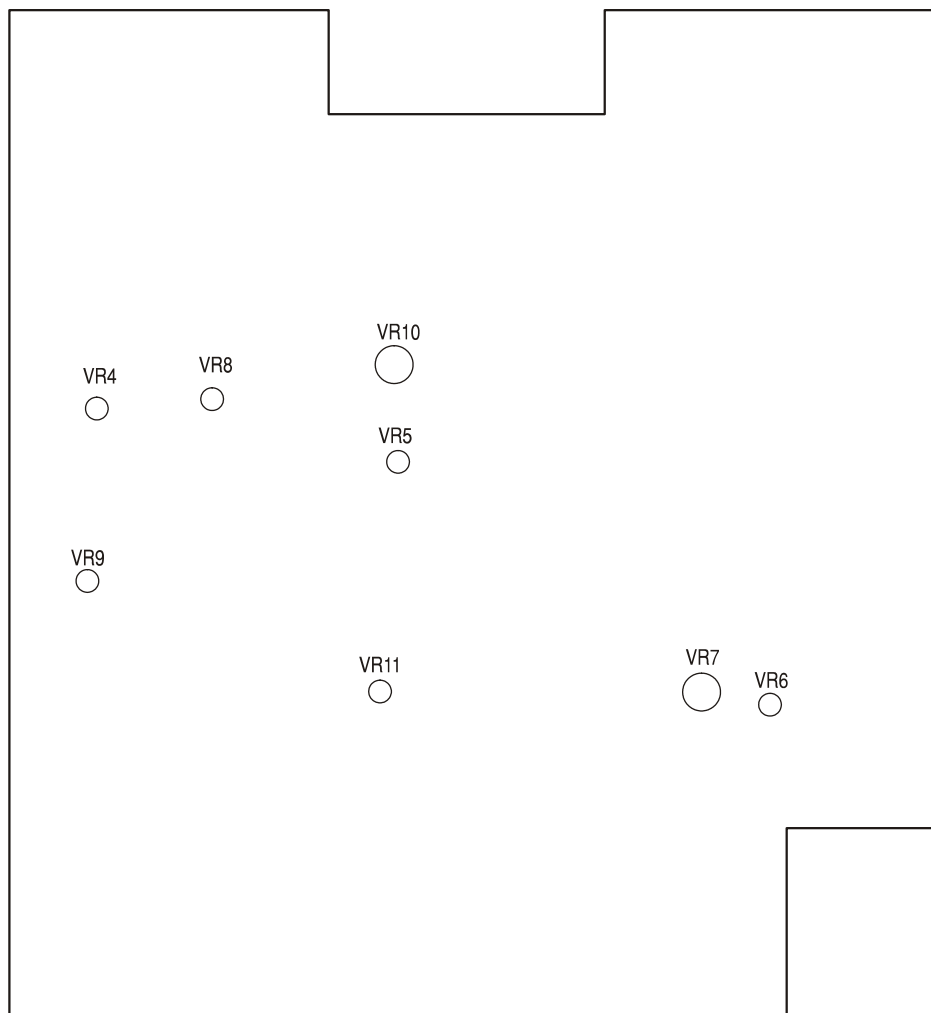
Control pcb calibration points (viewed from rear)
